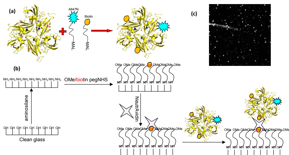
Figure 1: (a) K204C variant of SLAC conjugated with Atto647N–maleimide and biotin–PEG–maleimide. The conditions are chosen so that the dye–to–protein labeling ratio does not exceed 5 % to ensure most enzyme molecules carry only one or no fluorescence label. T1 Cu is depicted in blue, TNC in grey and Cys204 in red. (b) Functionalization of glass coverslips with aminosilane and PEG linkers and immobilization of SLAC conjugates using the NeutrAvidin–biotin interaction. (c) A 40x40 μm 2 image taken under a confocal fluorescence microscope of the sample prepared in (b). The bright spots are individual SLAC molecules. For details about conjugation, immobilization, and confocal setup, see Supplementary Information.
