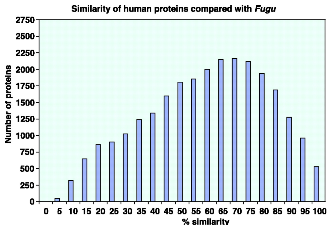
Figure 8. Distribution of protein similarities between Fugu and human proteomes. Global similarities were calculated as the sum of similarities in all nonoverlapping HSPs using a BLOSUM62 matrix, over the query (human) sequence length.
