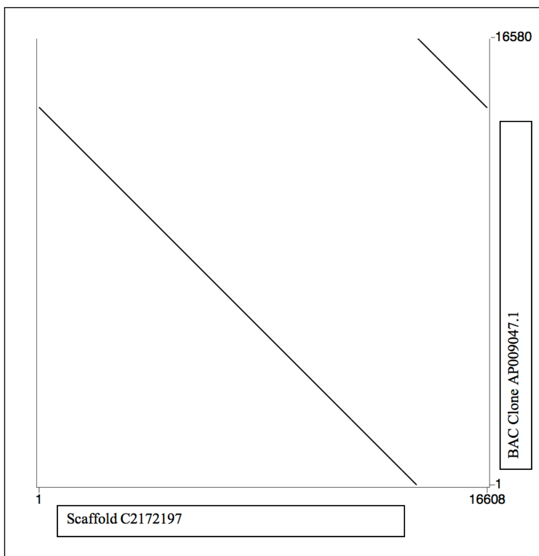
Figure 12 Figure showing the base by base alignment of Scaffold C2172197 and Clone of the mitochondrial genome (BAC Clone AP009047)
