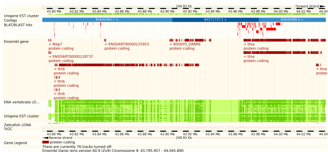
Figure 9 Scaffold24544 mapping to zebrafish chromosome 9 containing the Titin loci
