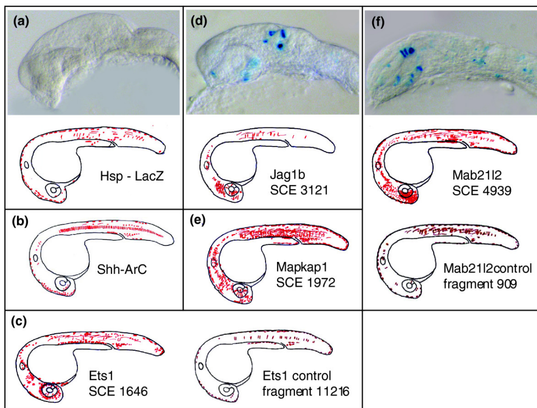
Figure 7 Expression profiles of X-Gal stained embryos. (a-f) Expression profiles of 1-day-old X-Gal stained zebrafish embryos. Each expression map represents a composite overview of the LacZ-positive cells of 65-175 embryos. Gene names and fragment/SCE id are shown. Detailed distribution of X-Gal stained cells in different tissues as well as data for all other fragments are shown in Table 3. Side view of head region of LacZ-stained embryos are shown with anterior to the left. (panel a) HSP-lacZ injected embryo. (d) Embryo co-injected with SCE 3121 associated with Jag1b gene. (f) Embryo co-injected with SCE 4939 associated with Mab21l2 gene. SCE, shuffled conserved region.
