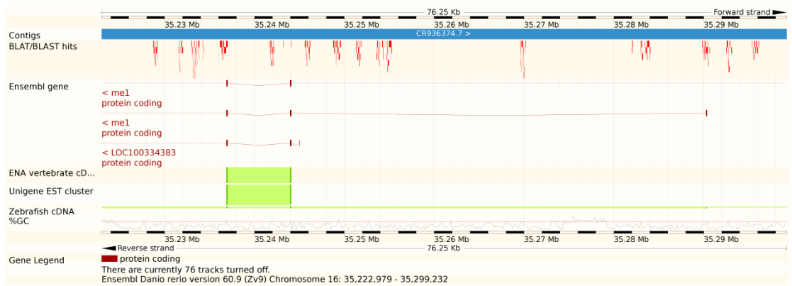
Figure 8 Scaffold8659 mapping to chromosome 16
