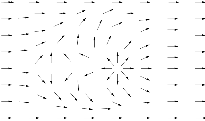
Figure 5.1: The destruction of the spin vortex by dipolar locking. The U(1) degree of freedom is indicated by an arrow. In the center where the electric field is located, the angle follows a vortex configuration of unit winding number, corresponding to one charge quantum. Since the electric field, decaying as \frac{1}{r} , is not able to compete with the dipolar locking at long distances, the U(1) angle becomes fixed at the Leggett angle, indicated by a horizontal arrow.
