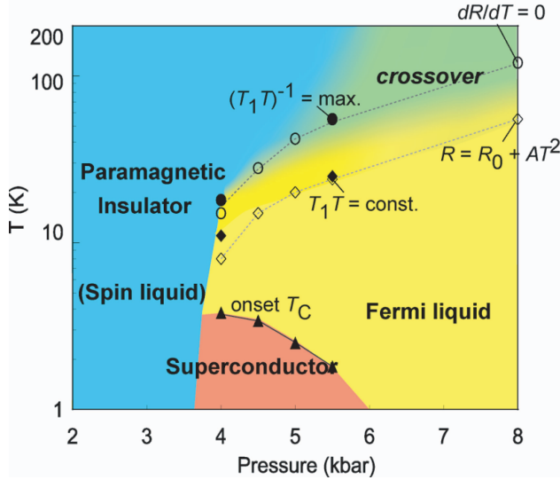
Figure 9.1: The phase diagram of the highly frustrated \kappa -(ET) 2 Cu 2 (CN) 3 , as proposed by Kanoda [38]. The spin liquid state shows linear specific heat, which might signal the presence of a spinon Fermi surface. This would amount to making a spinon Fermi liquid out of an insulator. Then the interesting possibility is that this spinon metal might be unstable against an S = 1 spin superfluid.
