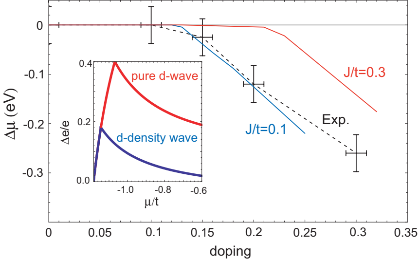
Figure 8.3: Chemical potential shift as a function of doping, showing the phase separation behaviour of the reformulated mean field theory. Indeed, the chemical potential starts to shift for appreciable dopings only. The blue line are the numerical results for J/t = 0.1 , and agrees very well with the experimental results from Fujimori [19] (dotted line). The red line depicts the results for J/t = 0.3 . The critical doping changes, but not the compressibility. The inset shows that ignoring a_0^1 , i.e., ignoring the s -wave component, gives a false vacuum. Indeed, there is a positive relative energy difference between the pure dSC and our mean field theory, growing with doping (red line). The inset also shows that for non-zero doping, the DDW/SFP state (blue line) is higher in energy than the superconducting states.
