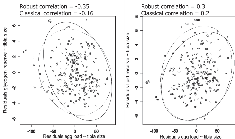
Fig.6: Classical and robust correlations between size-corrected egg load and size-corrected glycogen and fat reserves in Iranian Leptopilina boulardi . The data from the 11 populations have been pooled. Solid lines showed robust and dotted line classical correlation.
