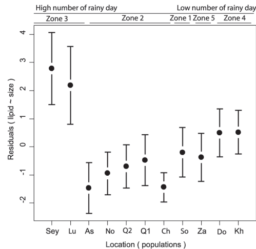
Fig.3: Lipid reserves in 11 Iranian populations of Leptopilina boulardi (values are residuals of the regression of lipid reserve on tibia length to correct the effect of size; error bar represent Standard Error). Populations are ordered according to their ranked number of rainy days per year (high to low). Correlation between lipid reserve and rainy days is significant after excluding first two populations ( t = -3.45 , P < 0.001 ).
