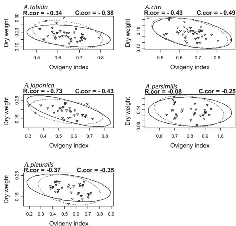
Fig.5: Within-species correlations between dry weight and ovigency index in five species of Asobara . Solid lines: robust correlation (R.cor). Dashed lines: classical correlation (C.cor).
