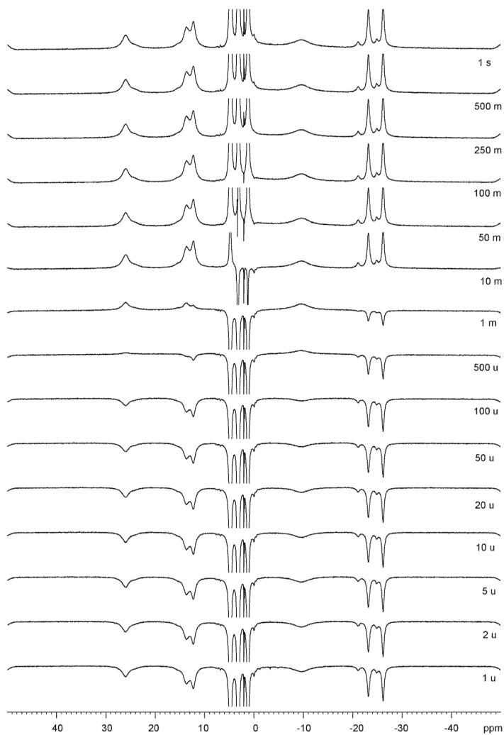
Figure 1: Inversion recovery pulse sequence NMR for the complex (\text{HNEt}_3) \text{ trans-}[\text{Mn}(\text{R-phoxCOO})(\text{S-phoxCOO})(\text{H}_2\text{O})_2] ( RS-5 ). (Chapter 3)
