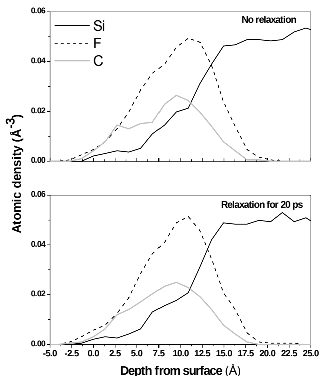
Figure 7: Atomic densities of the sample as a function of the depth for un-relaxed and relaxation of 20 ps after exposure to 20 ML \text{CF}_3 .
