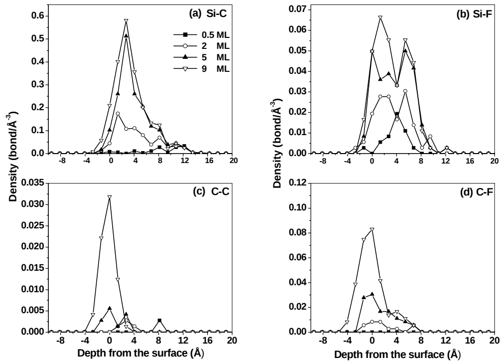
Figure 9: The Si-C, Si-F, C-C and C-F bond densities as a function of sample depth after different exposure times. The surface was bombarded by 50 eV CF for exposures equivalent to 0.5, 2, 5 and 9 ML.
