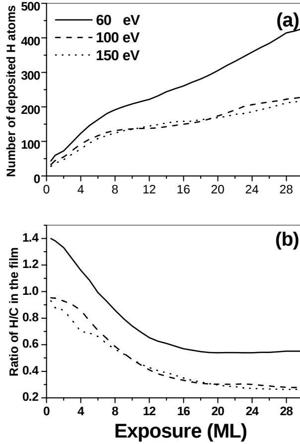
Figure 1: (a) Number of H atoms on the substrate as a function of exposure to \text{CH}_3 with incident energies of 60, 100 and 150 eV. (b) H/C ratio on the substrate as a function of exposure to \text{CH}_3 with incident energies of 60, 100 and 150 eV.
