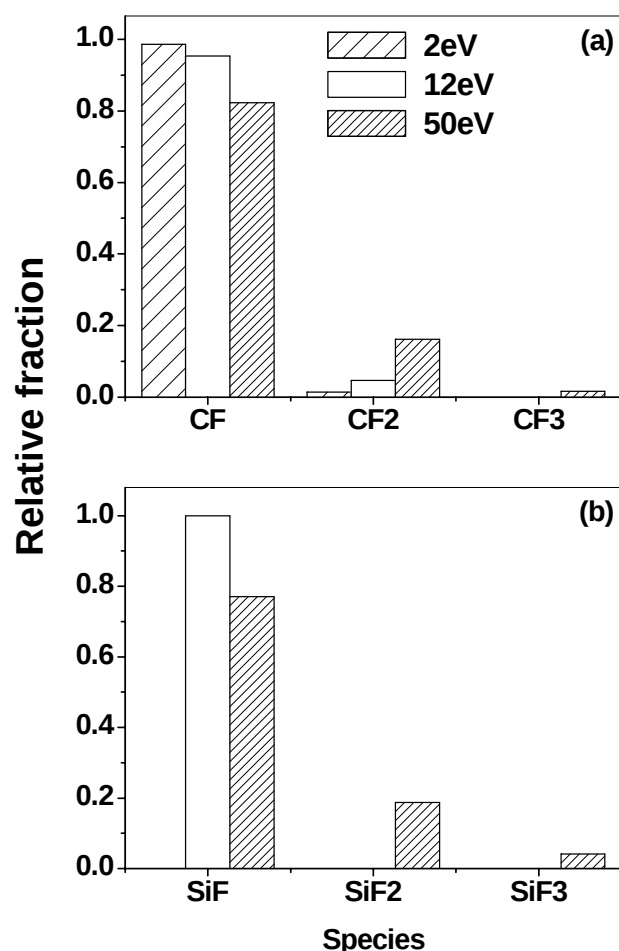
Figure 10: The relative fractions of (a) CF x and (b) SiF x (x=1-3) on the sample for 2, 12 and 50 eV bombardment of the sample. In each case the exposure was equivalent to 10 ML.
