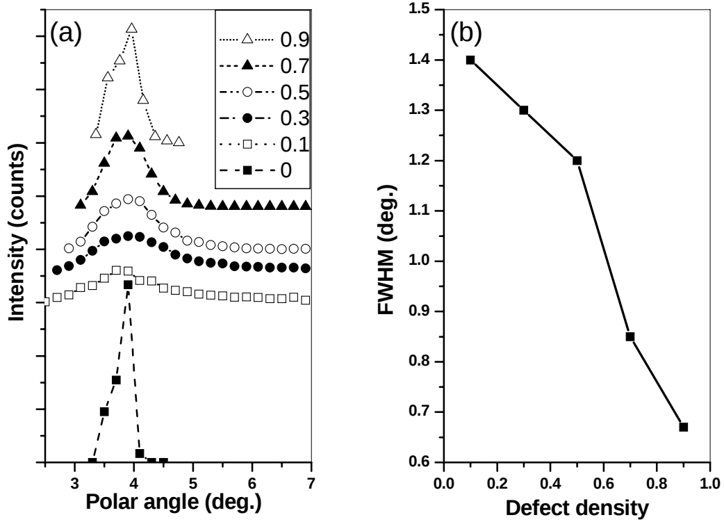
Figure 2: (a) Scattered distributions for 3 keV Ar as a function of the polar angle for different defect densities at 300 K (incident angle of 2^\circ ). (b) Full-width at half-maximum (FWHM) of the polar scattering distribution as a function of the adatom density.
