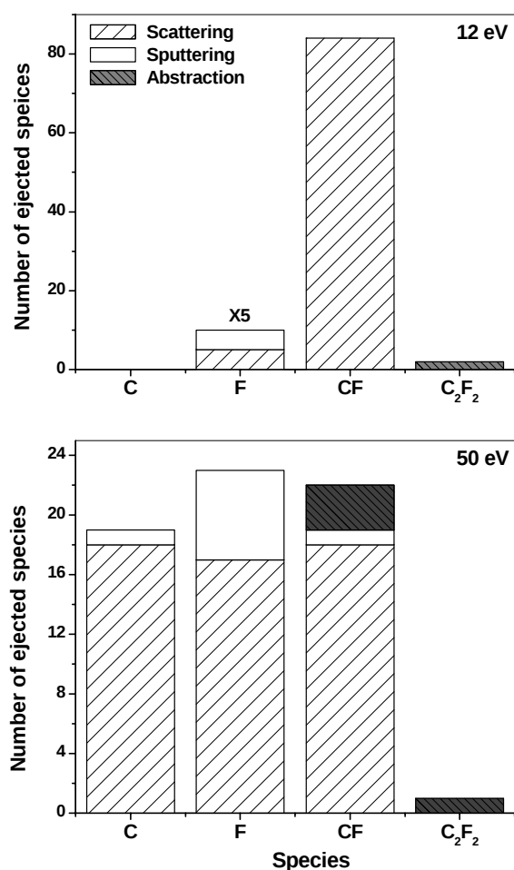
Figure 4: The cumulative yield of gas phase species that are ejected from the surface for 2, 12 and 50 eV after 10 ML exposure.
