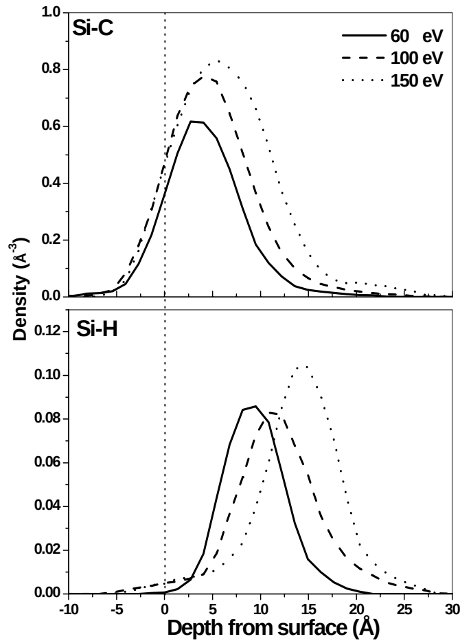
Figure 3: Bond density profiles of Si-C and Si-H as a function of substrate depth after exposure of Si(100) to the equivalent of 40 ML of \text{CH}_3 with incident energies of 60, 100
