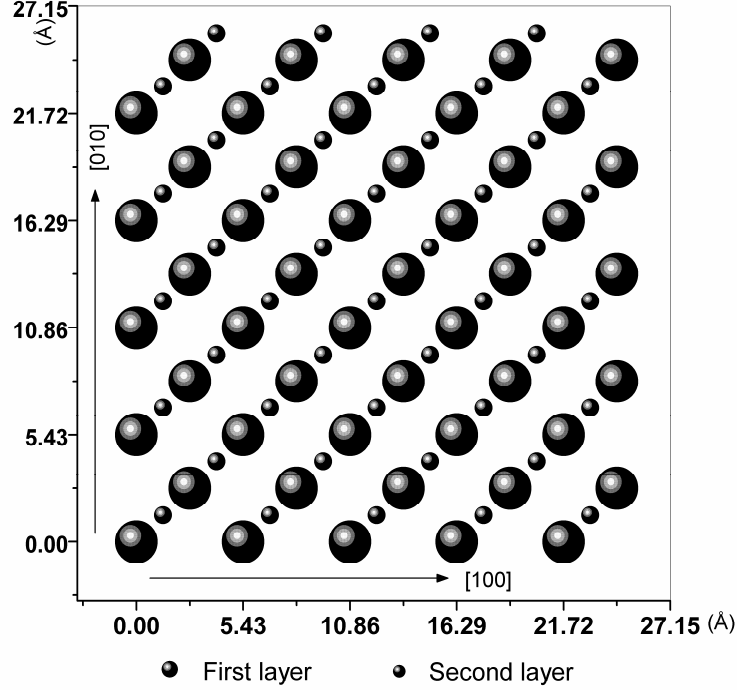
Figure 1: The top view of an unreconstructed \text{Si}(100) single crystal lattice, showing the relative positions of atoms in the first two layers.
