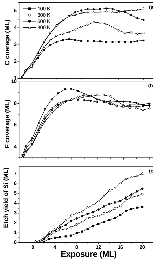
Figures 11: Coverages of (a) C and (b) F atoms on the sample as a function of exposure for different sample temperatures; (c) Si etching yield as a function of the exposure.
