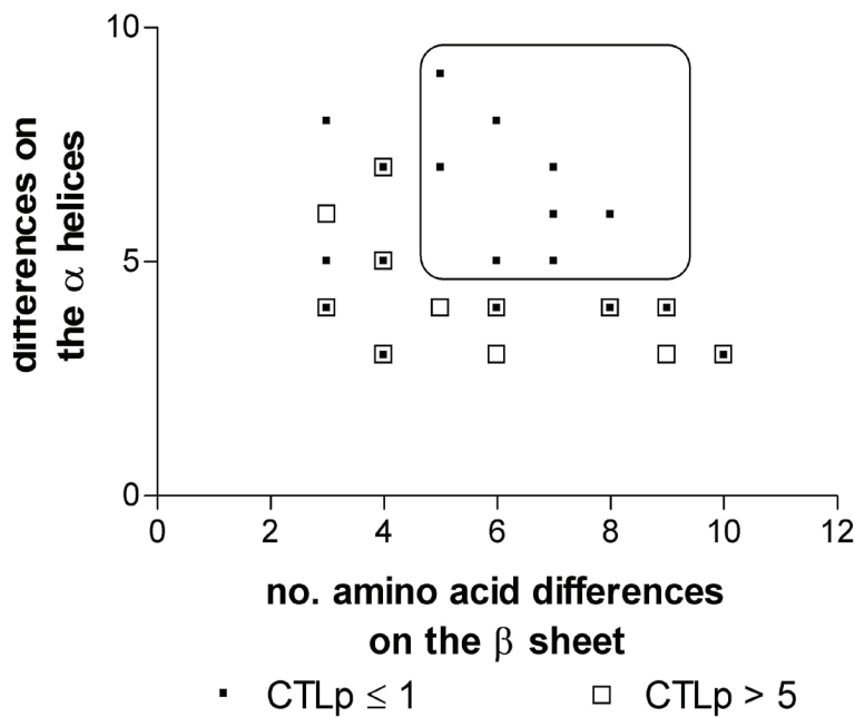
Figure 5: The number of amino acid differences in the \alpha helices and \beta sheet of HLA-C versus T cell alloreactivity in vitro (CTLp/10 6 PBL). The number of pairs in each group: 24 within the group with an undetectable CTLp frequency and 15 within the group with detectable CTLp frequency. Five or more differences in the \alpha helices and at least five differences in the \beta sheet lead to undetectable CTLp frequencies. Please note that certain pairs have similar numbers of amino acid differences on both \alpha helices and \beta sheet and thus overlap each other in this figure.
