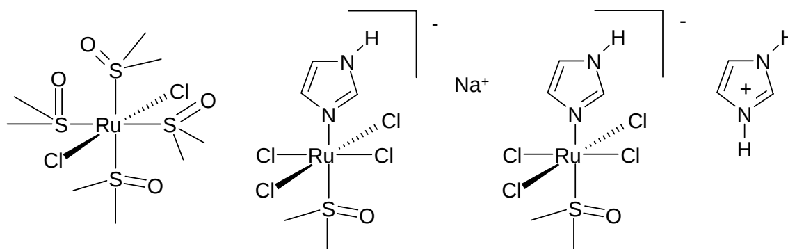
Fig.1.12. Dimethylsulfoxide complexes. From left to right, \text{trans}[\text{Ru}(\text{II})(\text{dmsO})_4\text{Cl}_2] , \text{Na}\{\text{trans}[\text{Ru}(\text{III})\text{Cl}_4(\text{dmsO})(\text{Him})]\} (NAMI) and [\text{H}_2\text{Im}]\{\text{trans}[\text{Ru}(\text{III})\text{Cl}_4(\text{dmsO})(\text{Him})]\} (NAMI-A).
