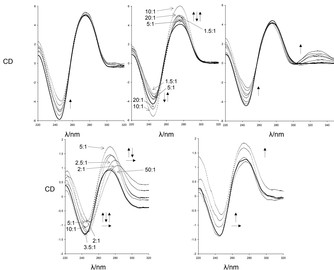
Fig.4.4. Above, circular dichroism spectra of ct-DNA 300 \mu M incubated for 24h with increasing concentrations of the mononuclear ruthenium complexes 1b (left), 1e (centre) and 1f (right). The DNA base pairs to ruthenium complex ratios are 20:1, 10:1, 5:1, 3:1, 2.5:1, 2:1 and 1.5:1. Below, CD spectra of ct-DNA 100 \mu M with increasing concentrations of the dinuclear complex 1g , from freshly-prepared samples (left) and from samples incubated for 24h (right). The DNA base pairs to ruthenium complex ratios are 50:1, 10:1, 5:1, 3.5:1, 2.5:1, and 2:1; the last two ratios were eliminated in the incubated sample because of precipitation. The solid line represents the ct-DNA; some of the curves are labelled with the base pairs to ruthenium complex ratios. The arrows in bold indicate a variation of the intensity of the band upon addition of ruthenium.
