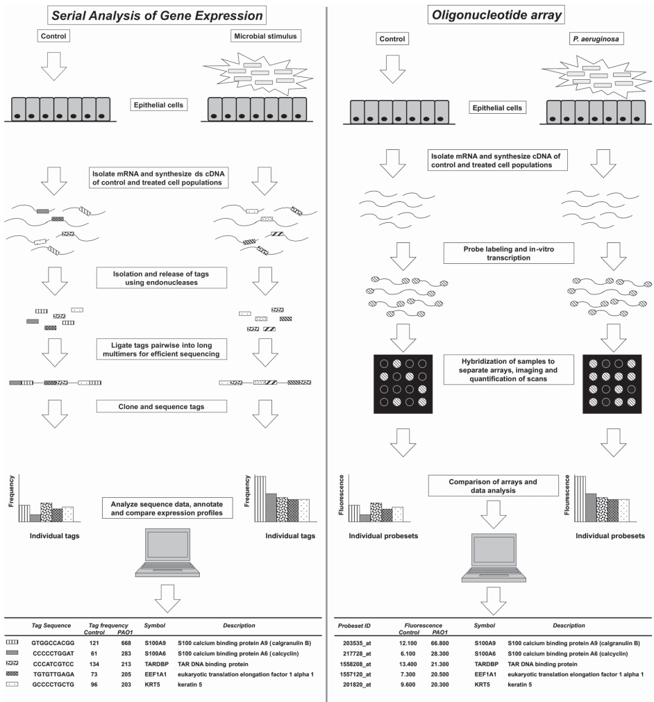
Figure 1: Outline of the SAGE and microarray technology. A flow-chart of the SAGE and microarray technologies is presented from top to bottom. In the first step, cultured cells are exposed to a pathogen. Isolated RNA is processed as such required for SAGE or microarray technology. Collected data reveals the expression profiles in the cells of interest under the studied conditions as illustrated in the lower table.
