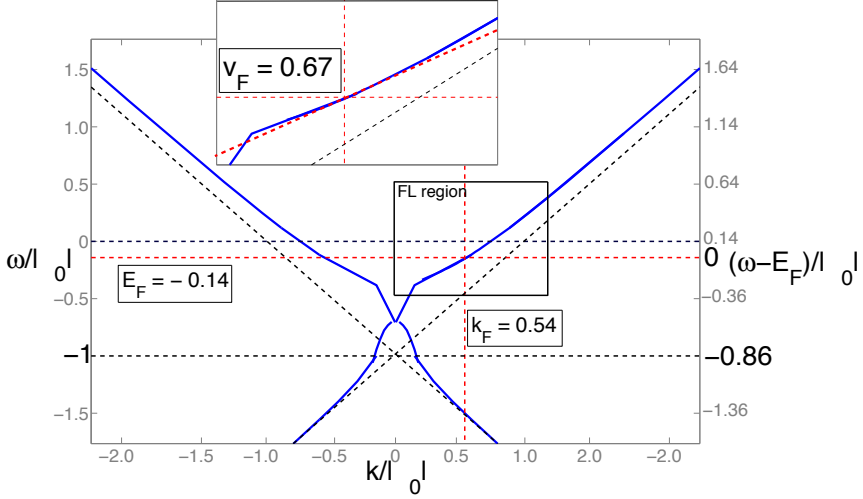
Figure 3.3: Maxima in the spectral function as a function of k/\mu_0 for \Delta_\Psi = 1.35 and \mu_0/T = -30.9 . Asymptotically for large k the negative k branch recovers the Lorentz-invariant linear dispersion with unit velocity, but with the zero shifted to -\mu_0 . The peak location of the positive k branch cut that changes into the quasiparticle peak changes significantly. It gives the dispersion relation of the quasiparticle near (E_F, k_F) . The change of the slope from unity shows renormalization of the Fermi velocity. This is highlighted in the inset. Note that the Fermi energy E_F is not located at \omega_{AdS} = 0 . The AdS calculation visualizes the renormalization of the bare UV chemical potential \mu_0 = \mu_{AdS} to the effective chemical potential \mu_F = \mu_0 - E_F felt by the low-frequency fermions.
