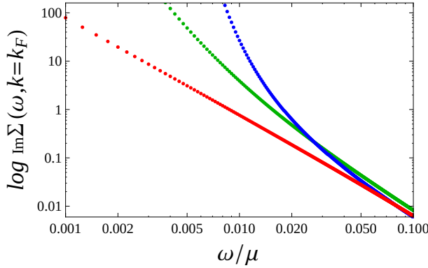
Figure 6.10: Imaginary part of the self-energy of the quasiparticle in the immediate vicinity of \omega = 0 for e = 5, 15, 50 (red, green, blue). It shows the crossover from power-law (solid line) (red line) to exponential. The self-energy of the quasiparticle undergoes a transition from quadratically damped peaks ( \Im\Sigma \sim \omega^2 , red points) toward exponentially narrow poles ( \Im\Sigma \sim e^{-1/\omega} , blue points). Notice that the all three peaks are stable: the power-law exponent is \nu = 1 with high accuracy, signalling a normal Fermi liquid phase.
