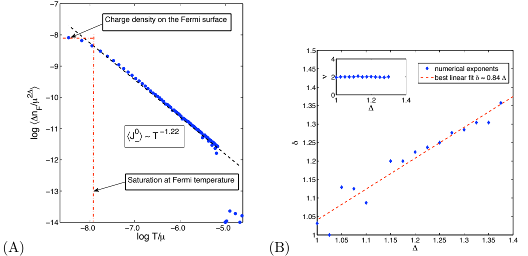
Figure 4.3: (A) Approximate power-law scaling of the Fermi liquid characteristic occupation number discontinuity \Delta n_F / \mu^{2\Delta} \sim T^{-\delta} as a function of T/\mu for \Delta = 5/4 . This figure clearly shows the saturation of the density at very low T/\mu . The saturation effect is naturally interpreted as the influence of the characteristic Fermi energy. (B) The scaling exponent \delta for different values of the conformal dimension \Delta . There is a clear correlation, but the precise relation cannot be determined numerically. The scaling exponent of the current I/\mu^{2\Delta+1} \sim T^{-1/\nu} obeys \nu = 2 with great accuracy, on the other hand (Inset).
