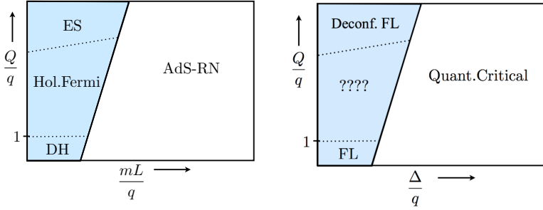
Figure 5.10: Schematic diagram of the different groundstate solutions of strongly coupled fermions implied by holography for fixed charge density Q . Here q is the constituent charge of the fermions and mL \sim \Delta the mass/conformal scaling dimension of the fermionic operator. One has the gravitational electron star (ES)/Dirac Hair (DH) solution for large/small Q/q and small mL/q dual a deconfined Fermi liquid/regular Fermi liquid in the CFT. For mL/q \sim \Delta/q large the groundstate remains the fermionic quantum critical state dual to AdS-RN.
