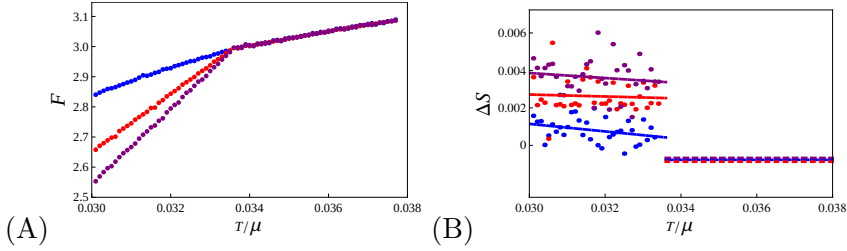
Figure 6.5: (A) Free energy (rescaled and centered to common value at the transition point) for the same parameters as in Fig. 6.4, in the vicinity of T = T_c ( not for the whole range of temperatures). The cusp characteristic of a first order transition is now clearly visible. The value of F on the RN side ( n = 0 ) is without error bars as the thermodynamic functions of the black hole can be exactly calculated. Notice how the slope of F in the low-temperature phase decreases as the number of levels increases: for N \rightarrow \infty we reach the electron star limit when the transition becomes continuous. (B) Difference between the entropy of the RN black hole and the entropy of the system \Delta S = S_{RN} - S , where entropy is obtained from free energy as S = -\partial F/\partial T , for the same parameters and in the same color schemes as in Fig. 6.4 and panel (A). The first order nature of the transition is recognized from the jump \Delta S at the critical point. Notice that the difference is positive for T < T_c , and thus the high temperature phase has more entropy as expected. The entropies in the RN/local quantum critical phase are exact, as they are calculated from the exactly known RN solution at given chemical potential. They are thus represented by a single (black) set of data points. The entropy is in relative (computational) units.
