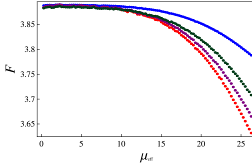
Figure 6.9: Free energy as a function of the fermion charge e in the crossover region for (\mu, m) = (2.2, 0.5) – red, (1.0, 0.5) – violet, (1.7, 1.0) – green and (1.7, 5.0) – blue curve and for a range of fermion charge values. On the abscise we plot the effective chemical potential \mu_{eff} = e\mu . The temperature is kept fixed at T = 0.0005 . All four cases exhibit a crossover about the same value of \mu_{eff}/T ( \mu_{eff}^{cross}/T \approx 20 ), suggesting that \mu_{eff} is indeed the key quantity that drives the changes of the Fermi surface. The low- \mu_{eff} region is a few-Fermi-surfaces DH-like system while the high- \mu_{eff} regime describes an ES-like multiplet of Fermi surfaces. We will later study in more detail the dispersion properties of the two regimes. Apart from the gradual and soft nature of the transition as seen from the numerical curves, the crossover (as opposed to phase transition) nature of the phenomenon also follows from analytical considerations. The dependence of the solution (f(z), h(z), \Phi(z)) on the parameters of the system (\mu, q, m) is analytical, which strongly suggests that the derivatives of the free energy \partial^k F / \partial \mu^k are continuous to all orders k = 2, 3, \dots
