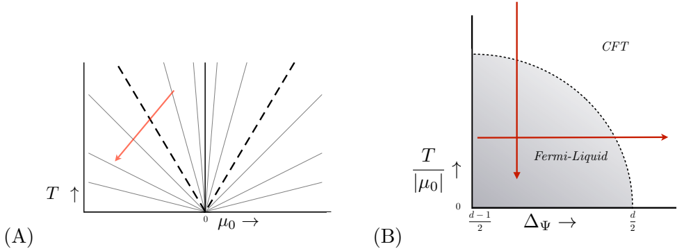
Figure 3.1: The phase diagram near a quantum-critical point. Gray lines depict lines of constant \mu_0/T : the spectral function of fermions is unchanged along each line if the momenta are appropriately rescaled. As we increase \mu_0/T we crossover from the quantum-critical regime to the Fermi-liquid. (B) The trajectories in parameter space (\mu_0/T, \Delta_\Psi) studied here. We show the crossover from the quantum critical regime to the Fermi liquid by varying \mu_0/T keeping \Delta_\Psi fixed; we cross back to the critical regime varying \Delta_\Psi \rightarrow d/2 for \mu_0/T fixed. The boundary region is not an exact curve, but only a qualitative indication.
