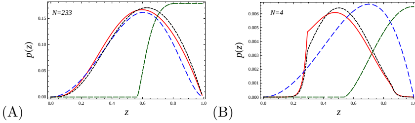
Figure 6.2: Comparison between full quantum pressure (dashed blue lines, Eq. 6.3.58) and thermodynamic pressure (solid red lines, Eq. 6.3.59) for two sets of parameters: (\mu, e, m) = (1.7, 100, 0.1) (A) and (\mu, e, m) = (1.7, 5, 1) (B). For comparison we plot also the fluid pressure p = en\Phi/2 (dashed green lines). Expectedly, all three models are close to each other for large N while for N small the level spacing is large and it is necessary to sum the contributions of individual levels: both the thermodynamic approximation and the simple fluid approximation deviate considerably from the exact sum.
