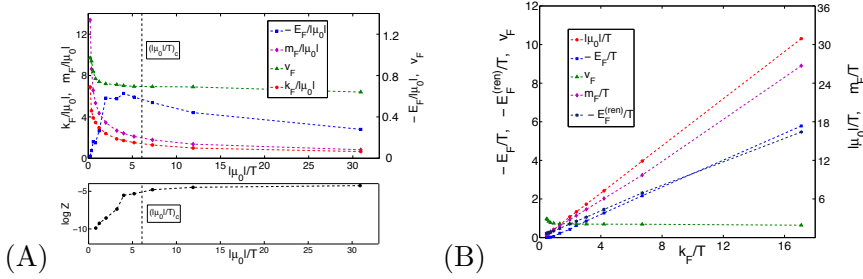
Figure 3.5: The quasiparticle characteristics as a function of \mu_0/T for \Delta_\Psi = 5/4 . Panel (A) shows the change of k_F, v_F, m_F, E_F and the pole strength Z (the total weight between half-maxima) as we change \mu_0/T . Beyond a critical value (\mu_0/T)_c we lose the characteristic T^2 broadening of the peak and there is no longer a real quasiparticle, though the peak is still present. For the Fermi-liquid k_F/T rather than \mu_0/T is the defining parameter. We can invert this relation and panel (B) shows the quasiparticle characteristics as a function of k_F/T . Note the linear relationships of m_F, E_F to k_F and that the renormalized Fermi energy E^{(ren)} \equiv k_F^2/(2m_F) matches the empirical value E_F remarkably well.
