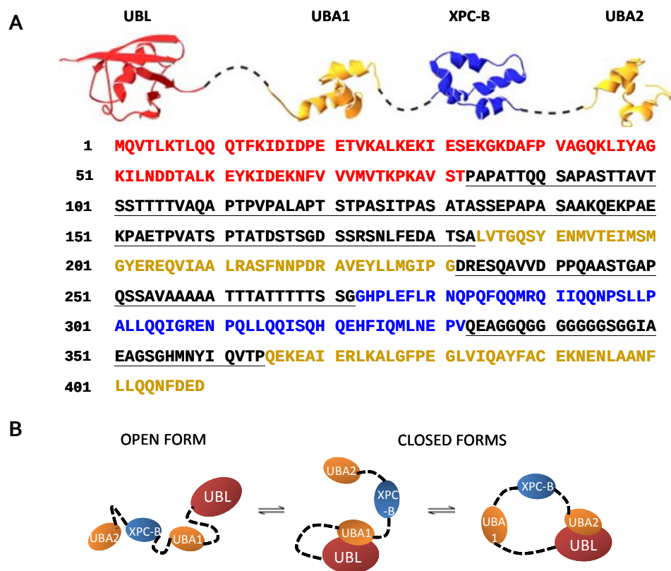
Figure 1: Schematic presentation of hHR23B protein.
