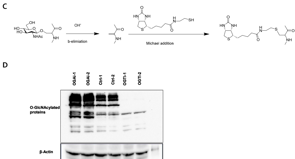
Figure 2: Chemical tools used in this chapter for O-GlcNAcylation study.
