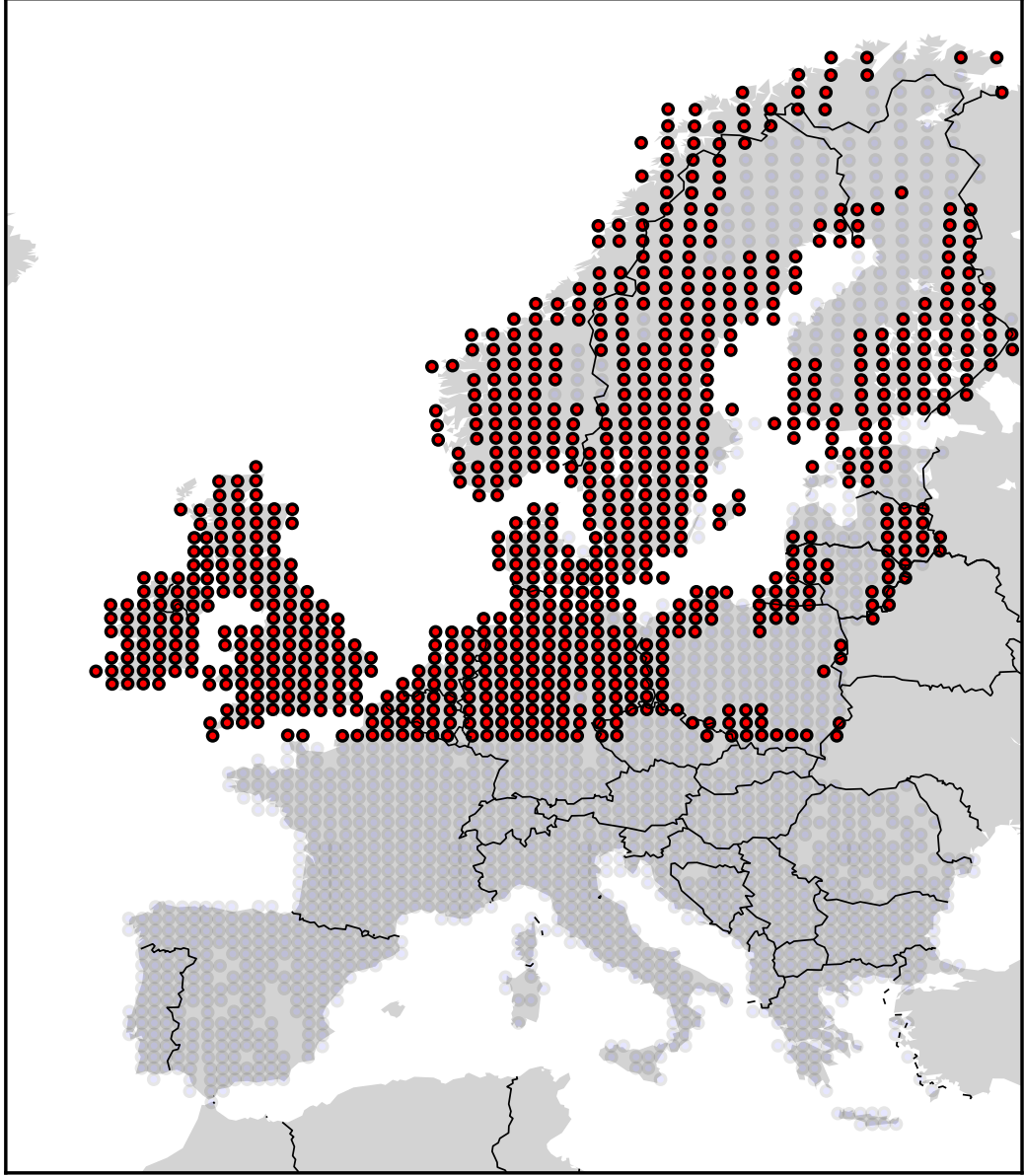
Figure 6.5: Regions in Europe that belong to the subgroup corresponding to D_{10} : \text{latitude} \geq 49.85 \wedge \text{prec\_feb} \geq 28.75 ( |G_{10}| = 839 ).
