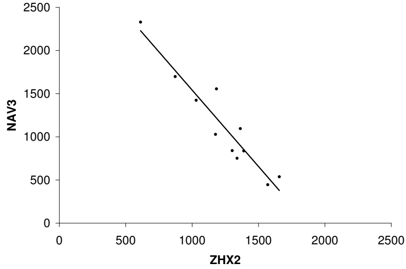
(a) G_2 , with \hat{r} = -0.950 .
