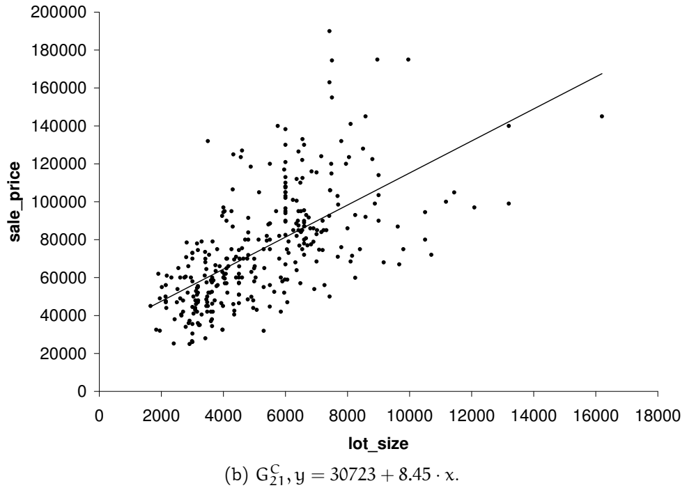
Figure 7.2: Windsor Housing - \varphi_{ssd} : Scatter plot of lot_size and sales_price for the subgroup corresponding to D_{21} : drive = 1 \wedge basement = 0 \wedge nbath \leq 1 and its complement.
