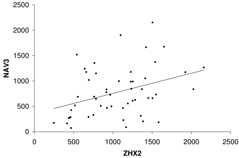
(b) G_2^C , with \hat{r} = 0.363 .
