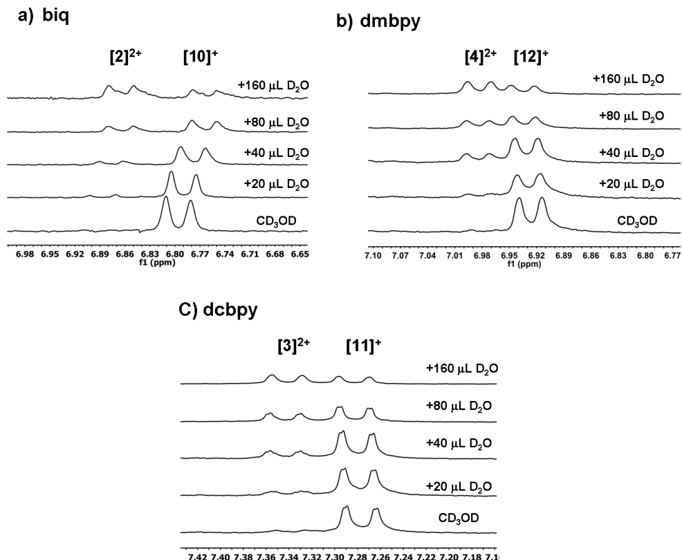
Figure AIII.3. ^1\text{H} NMR spectra showing the hydrolysis of [\text{Ru}(\text{terpy})(\text{N-N})(\text{Cl})]\text{Cl} ( [10]\text{Cl} , [11]\text{Cl} , and [12]\text{Cl} ) upon addition of increasing amount of \text{D}_2\text{O} in \text{MeOD} . Conditions: a) initial [\text{Ru}]_{\text{tot}} = 6.6 \times 10^{-3} \text{ M} , b) initial [\text{Ru}]_{\text{tot}} = 9.2 \times 10^{-3} \text{ M} , and c) initial [\text{Ru}]_{\text{tot}} = 9.6 \times 10^{-3} \text{ M} , T = 297 \text{ K} .
