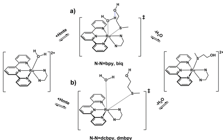
Scheme 3.3. The proposed transition states for the substitution of the aqua ligand in [Ru(terpy)(N-N)(H_2O)]^{2+} by Hmte, where a) N-N = \text{bpy, biq} (more compact transition state with hydrogen-binding contributing to a loose hepta-coordinated transition state) and b) N-N = \text{dcbpy, dmbpy} (less compact transition state).
