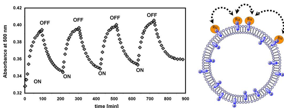
Figure 2.7. Left: Time evolution of the absorbance at 500 nm of an equilibrated solution initially containing DMPG vesicles functionalized with 35 mol% of ligand 4 and 5 mol% of [1](PF_6)_2 . At t=0 the sample is alternatively irradiated with blue light ( \lambda_e=465 nm, ON) or left in the dark (OFF). Right: representation of the light-induced hopping of a Ru complex on DMPG lipid bilayer. Conditions: T = 308 K, [lipid]_{tot} = 1.3 mM (as liposomes), vesicle average size= 140 nm, total concentration [Ru]_{tot} = 6.7 \times 10^{-2} mM, spectra measured every 3 minutes, photon flux \sim 3.9 \times 10^{-9} Einstein \cdot s^{-1} . Absorbance baseline due to light scattering at the vesicles was removed.
