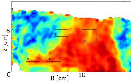
FIGURE 6.22: Indication of the location of regions A, B, C and D where we will monitor the alignment of the particles. The color represents s , which is the largest eigenvalue of T .
