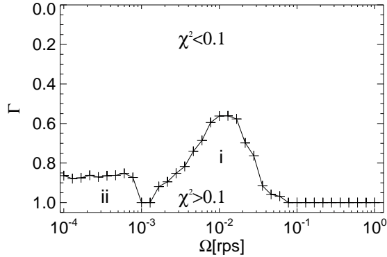
FIGURE 3.9: The boundary of \chi^2 = 0.1 , where we interpolate \chi^2(L) to find the location of the boundary. The two distinct regions where the data does not agree with T_f(H) (i and ii) can clearly be seen. In the next sections we will see what causes the deviations from the frictional model in these two regimes.
