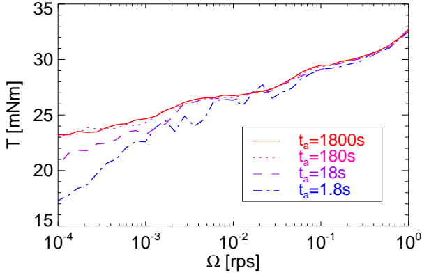
FIGURE 3.2: Flow curves for different averaging times t_a . Below \Omega \approx 0.5 \times 10^{-3} rps, the torque increases with the waiting time. The measurements are for \Gamma = 0.6 and h = 0.56 .
