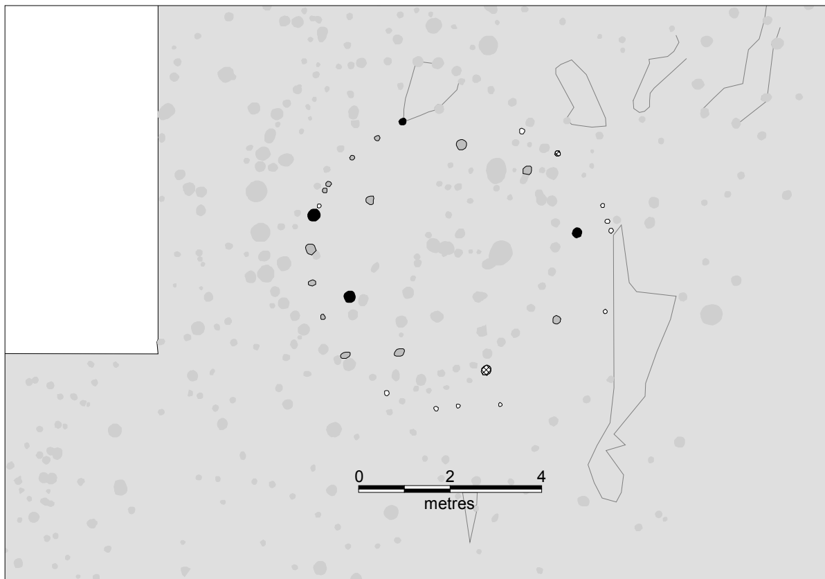
Figure 103. Structure 20.
