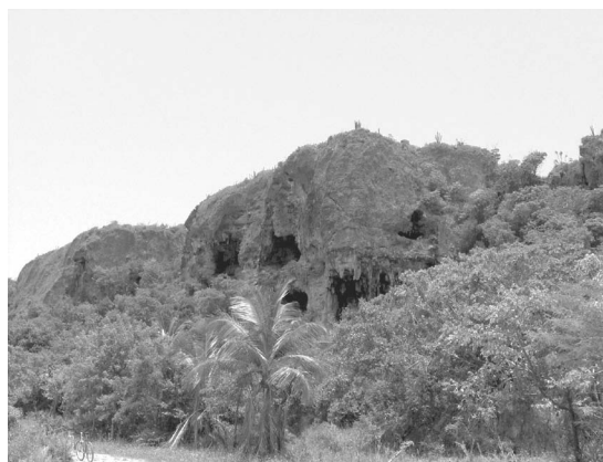
Figure 15. Flank margin caves en route to El Cabo. Note collapsed face exposing the void and speleothems which formed inside.
