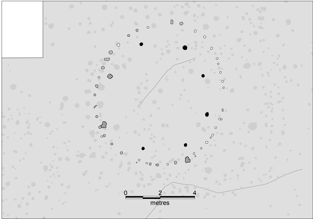
Figure 95. Structure 13.
