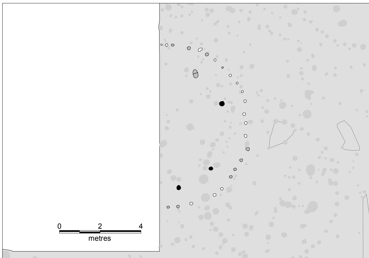
Figure 104. Structure 21.
