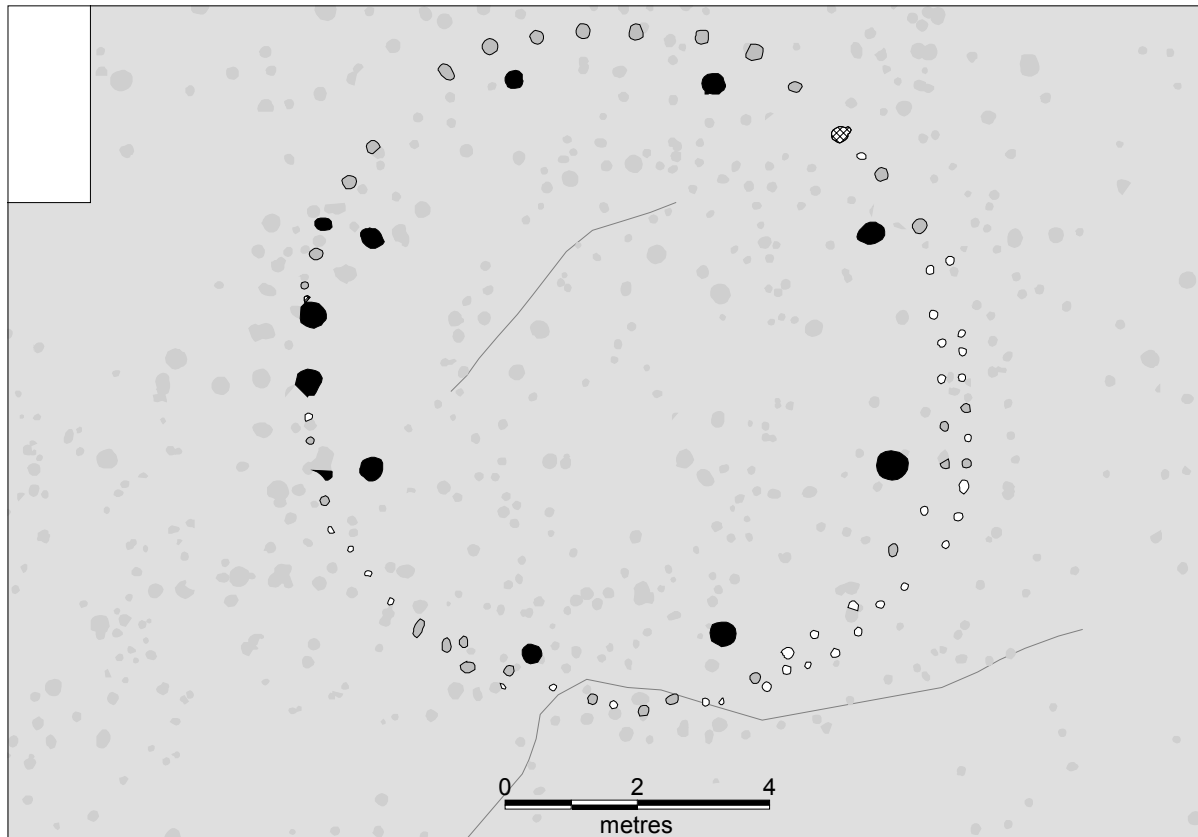
Figure 86. Structure 4.
