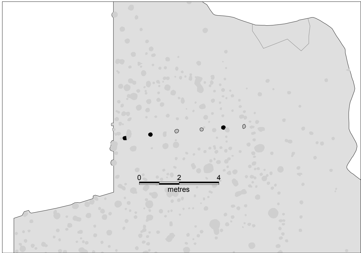
Figure 119. Structure 37.
