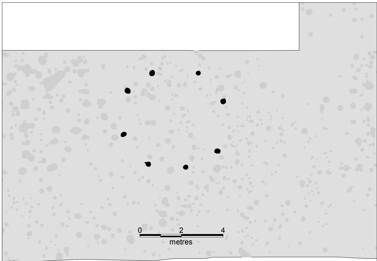
Figure 111. Structure 28
