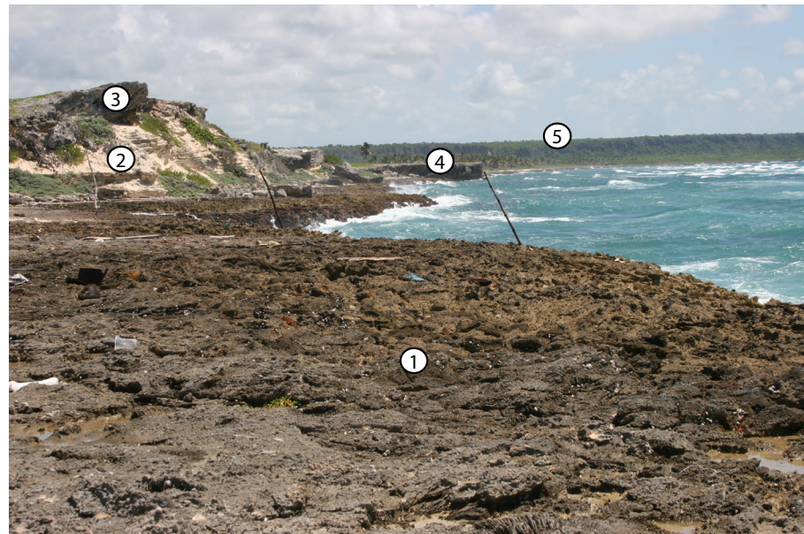
Figure 16. The local landscape of El Cabo showing aspects of its geomorphology. (1) coral limestone, (2) sand layer of intercalated deposits of former lagoon, (3) bedded limestone of intercalated deposits of former lagoon, (4) ibid. ; extending to the promontory of El Cabo, (5) limestone terrace of the cliffs behind El Cabo.
