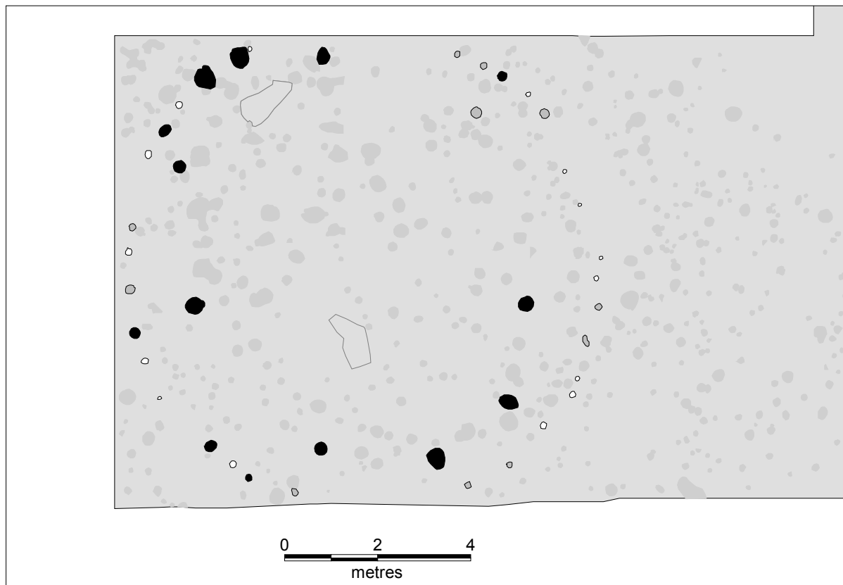
Figure 105. Structure 22.
