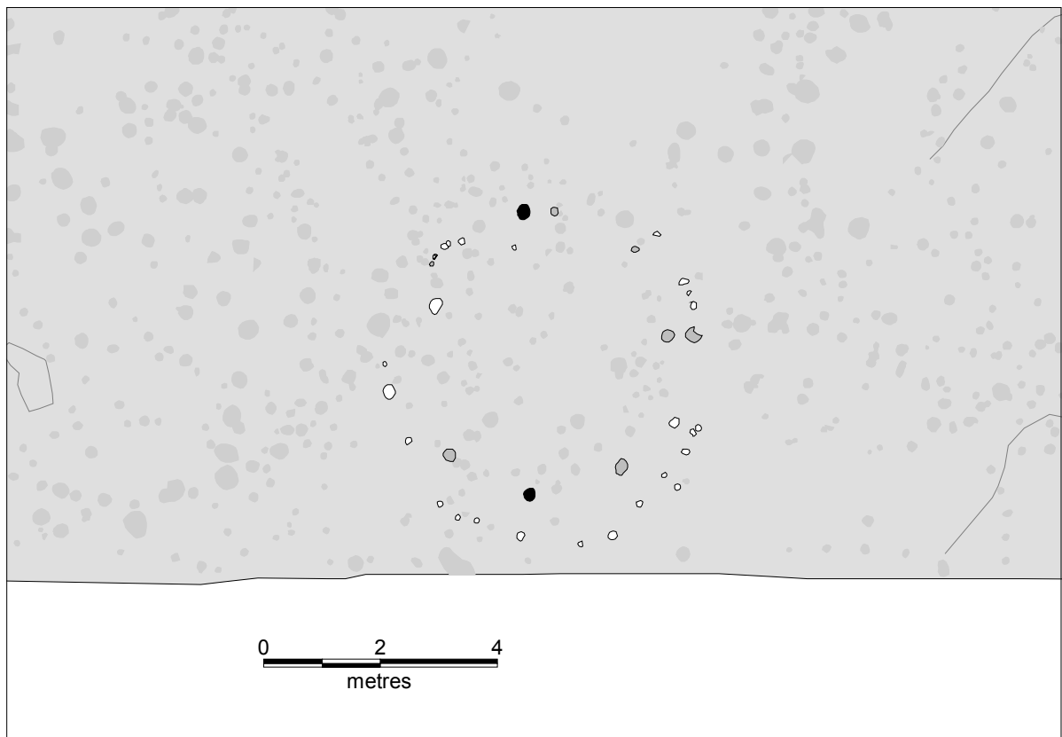
Figure 125. Structure 43.
