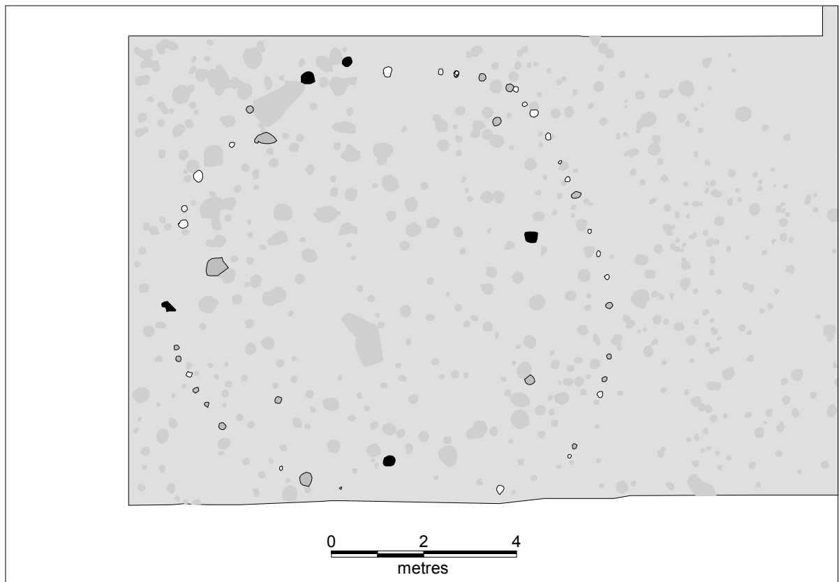
Figure 110. Structure 27.
