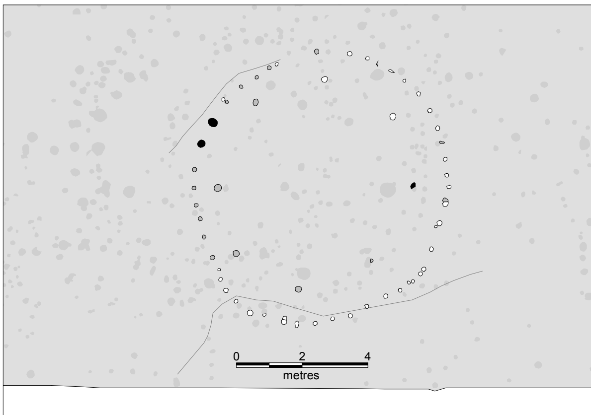
Figure 93. Structure 11.
