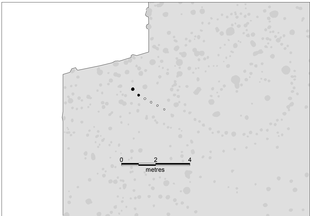
Figure 102. Structure 19.
