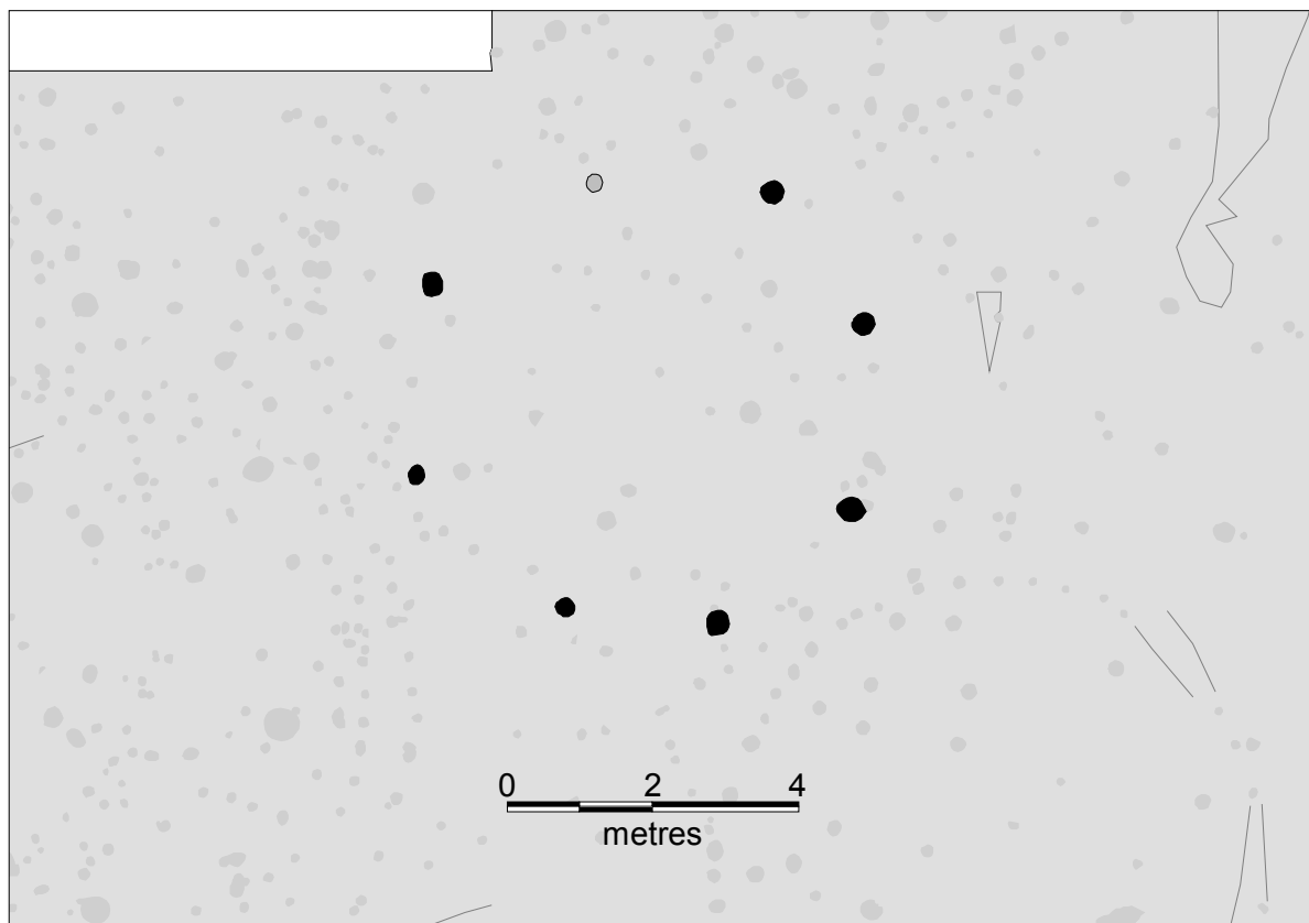
Figure 92. Structure 10.
