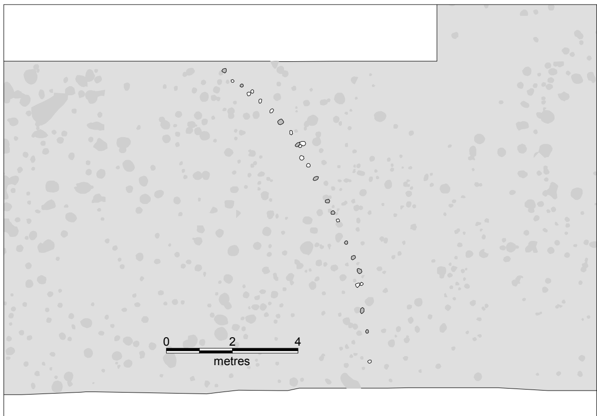
Figure 100. Structure 17.
