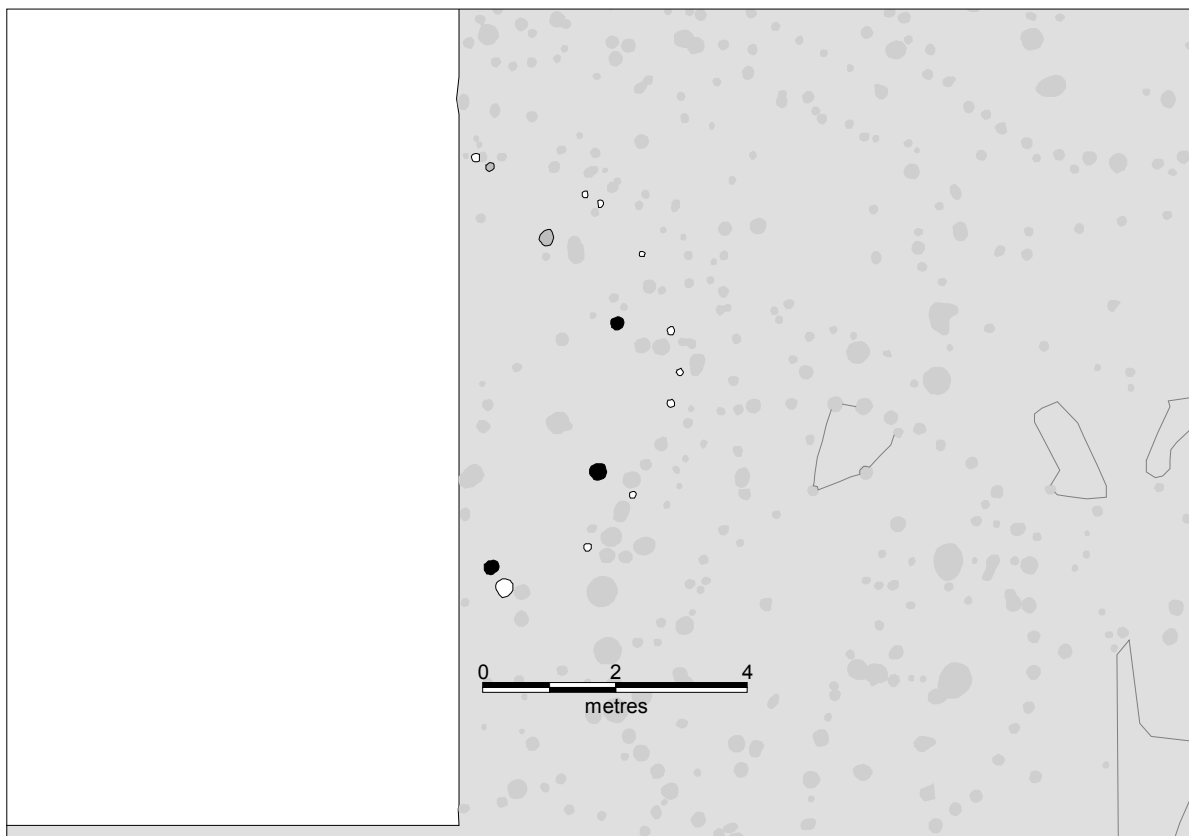
Figure 120. Structure 38.
