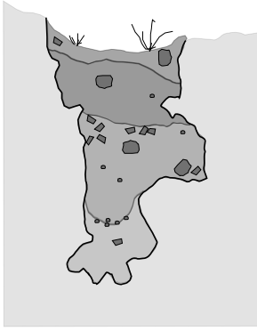
Figure 14. Dissolution pit filled with weathered rock and soil from various filling events (Adapted from Mylroie and Carew 1995). Size of pits ranges from a few centimetres to several metres.
