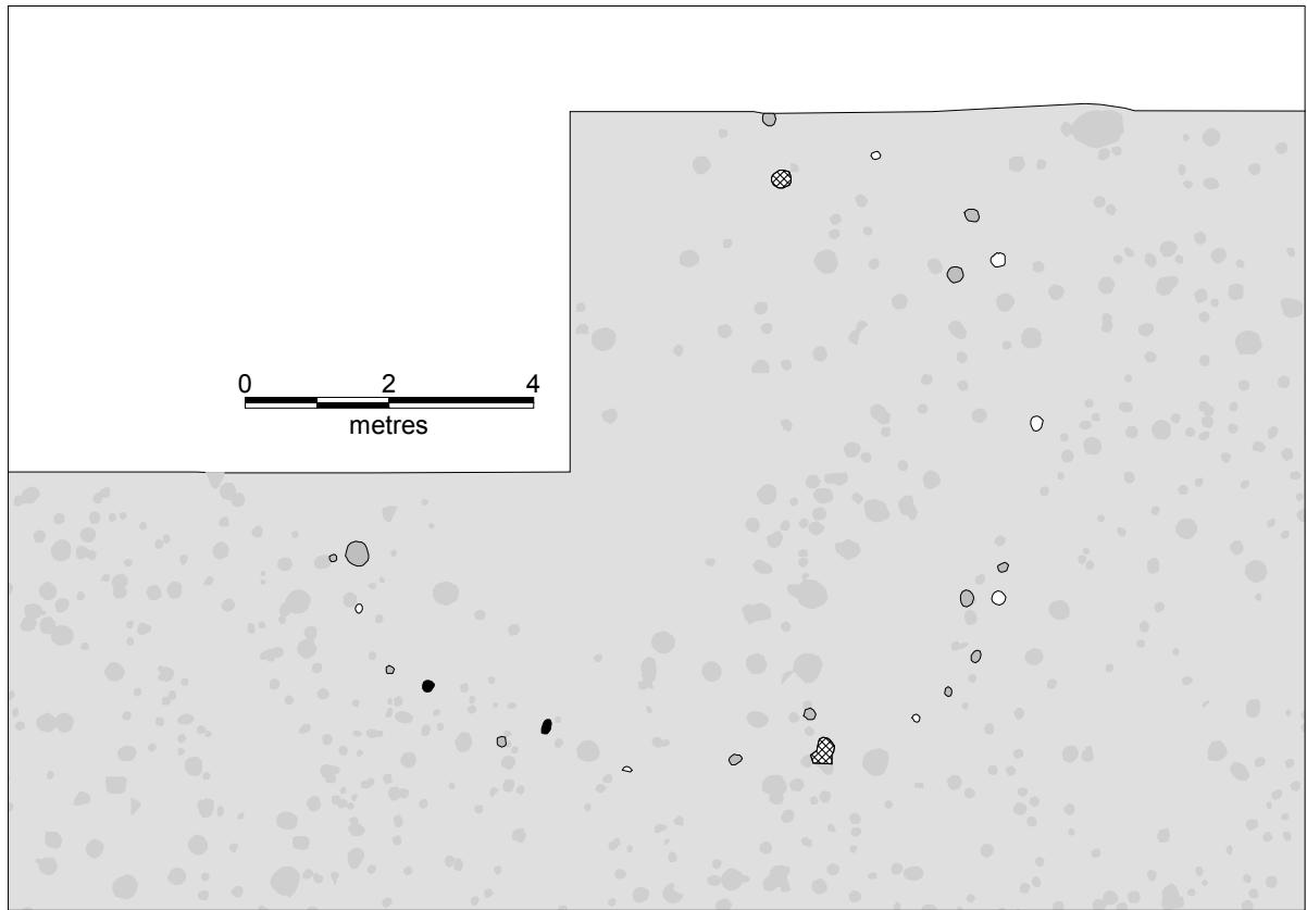
Figure 126. Structure 44.
