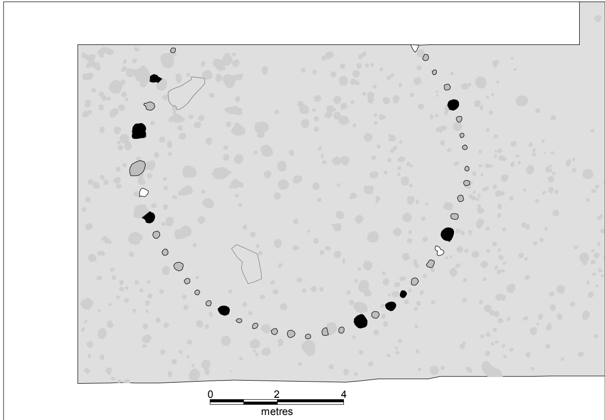
Figure 88. Structure 6.
