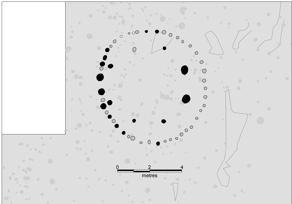
Figure 83. Structure 1.
