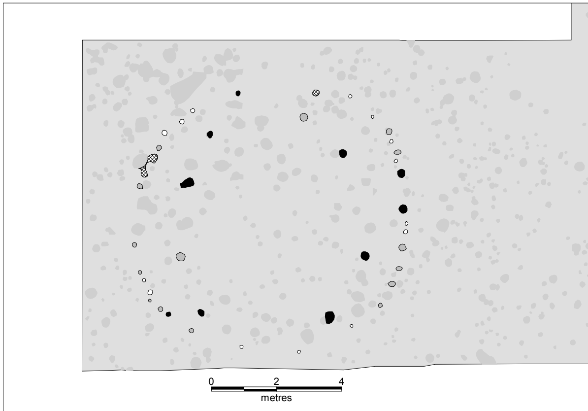
Figure 124. Structure 42.
