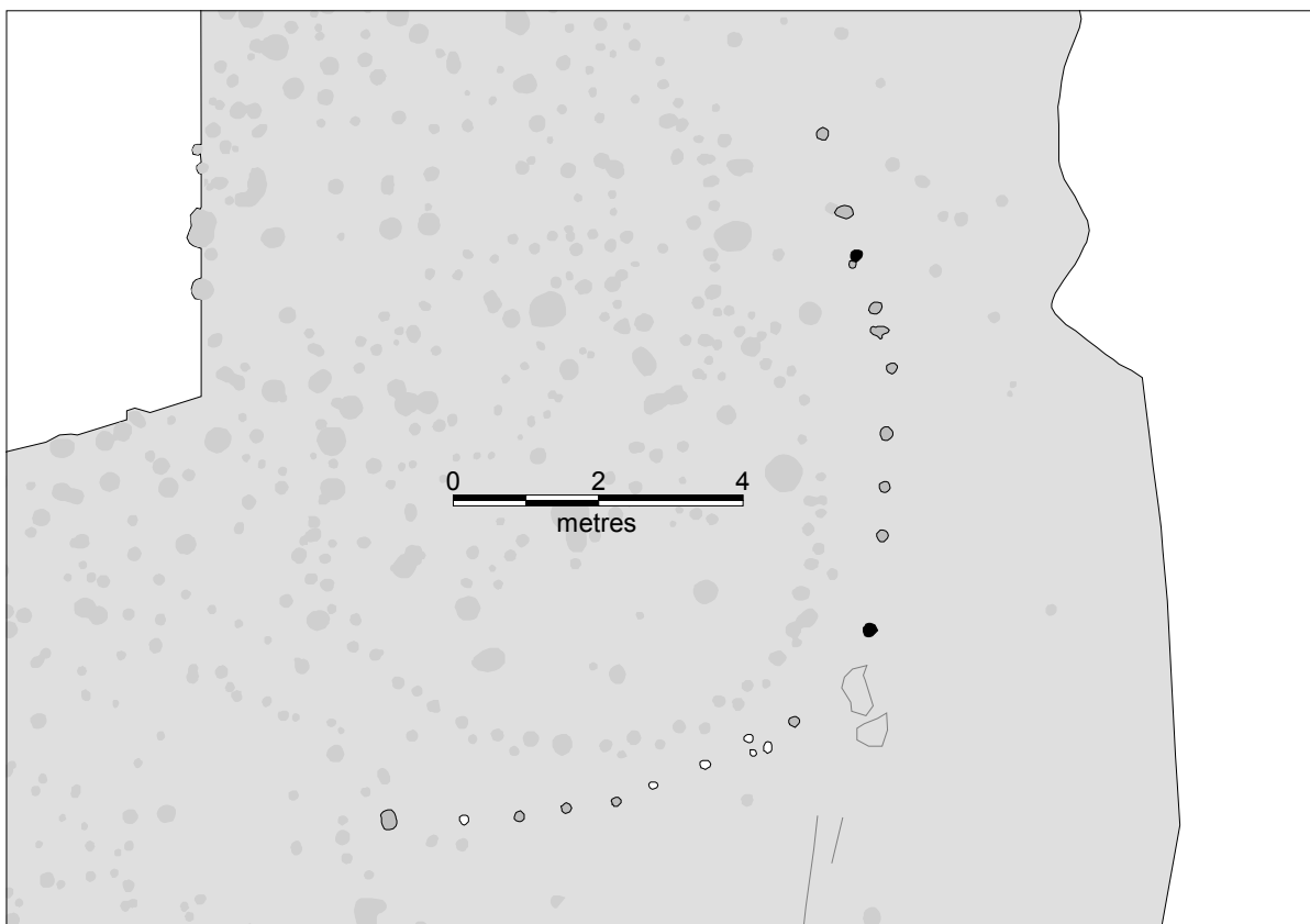
Figure 101. Structure 18.
