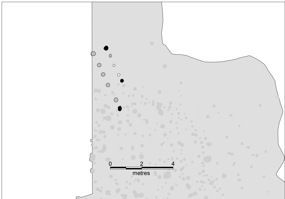
Figure 118. Structures 35 and 36.
