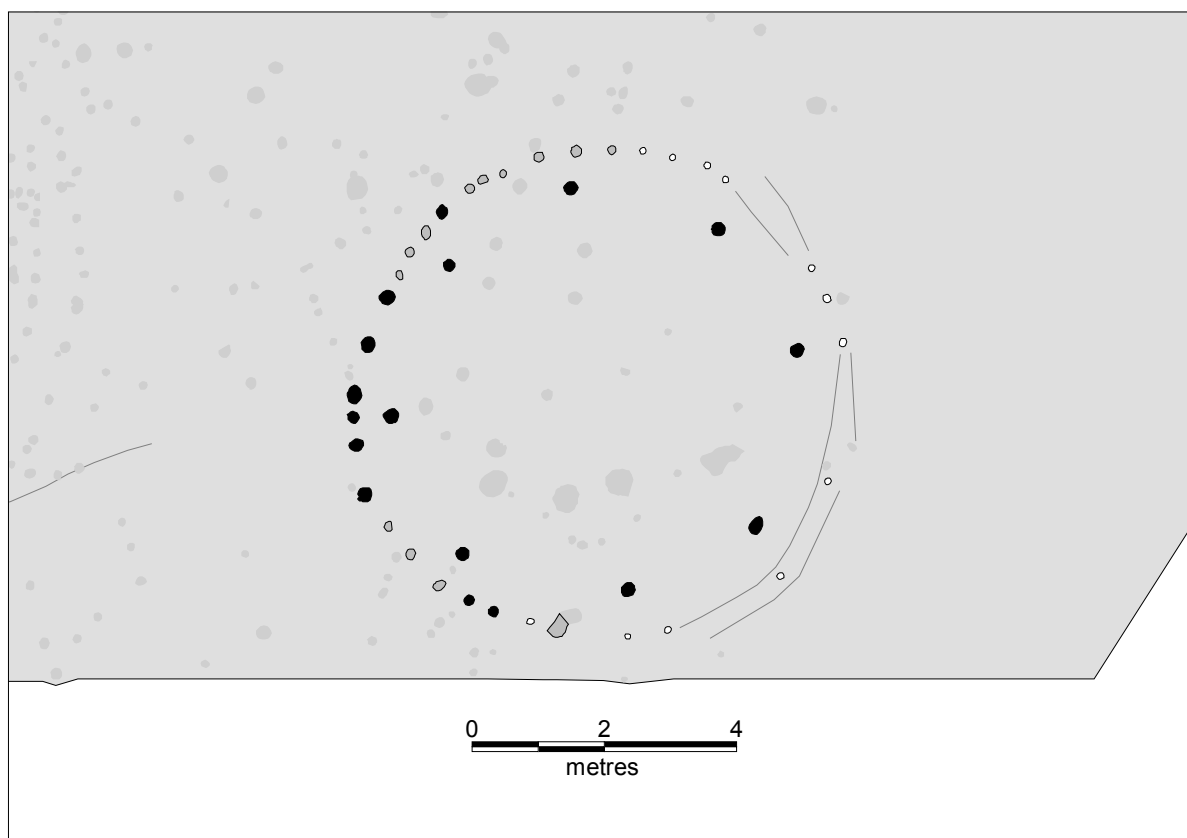
Figure 84. Structure 2.
