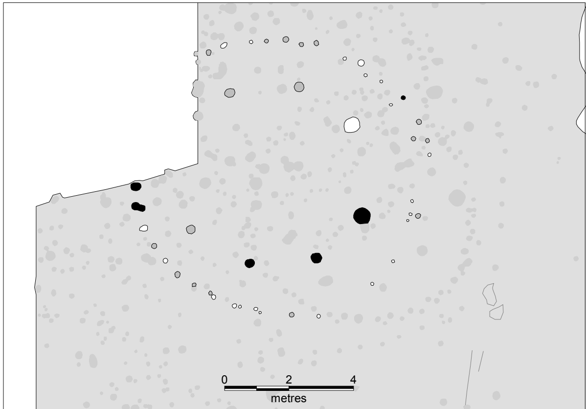
Figure 113. Structure 30.
