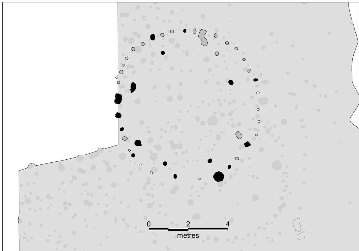
Figure 107. Structure 24.
