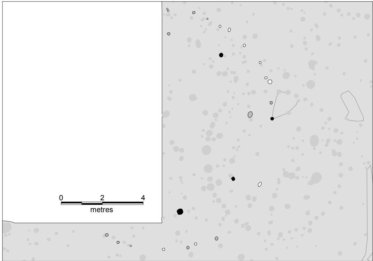
Figure 122. Structure 40.
