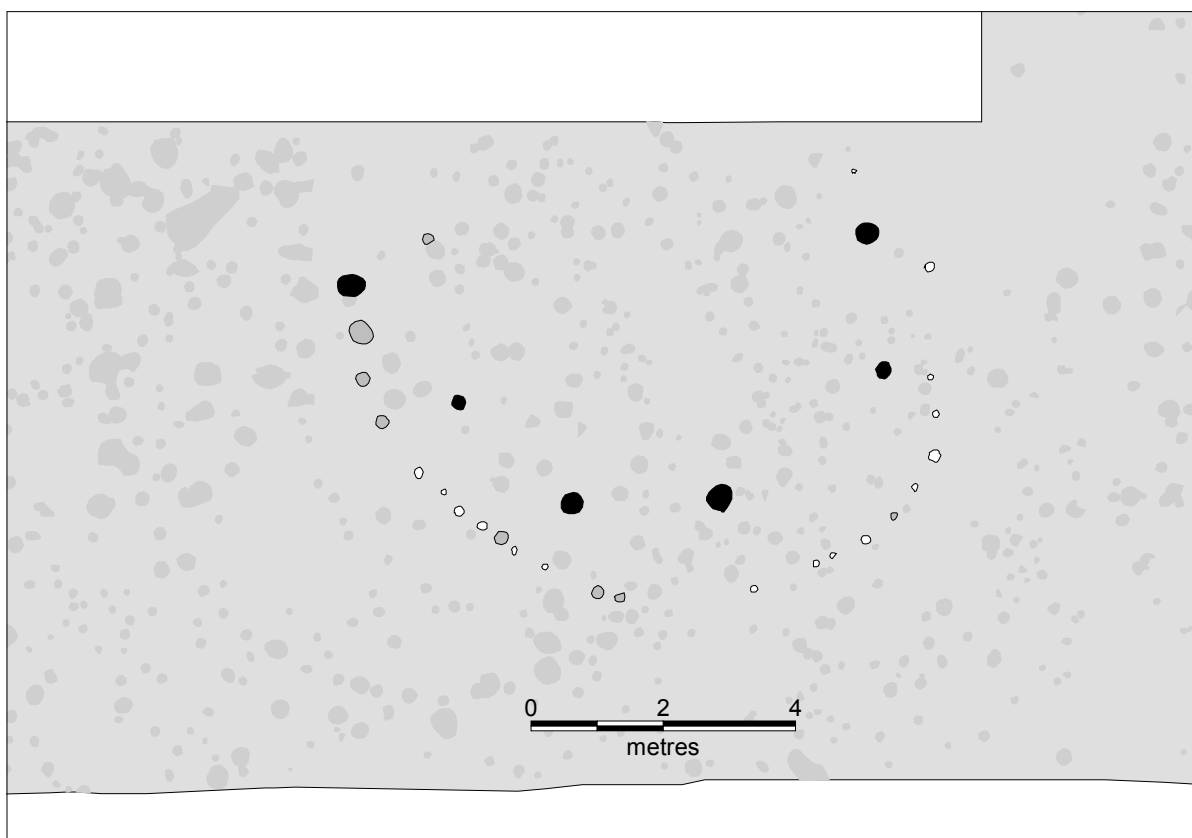
Figure 130. Structure 48.
