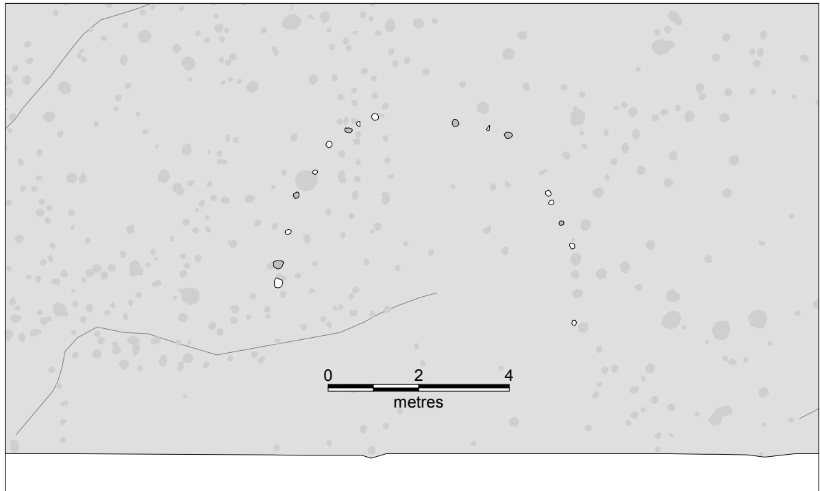
Figure 128. Structure 46.
