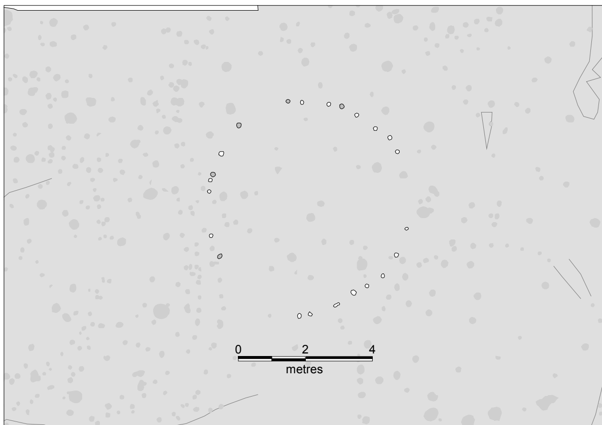
Figure 94. Structure 12.
