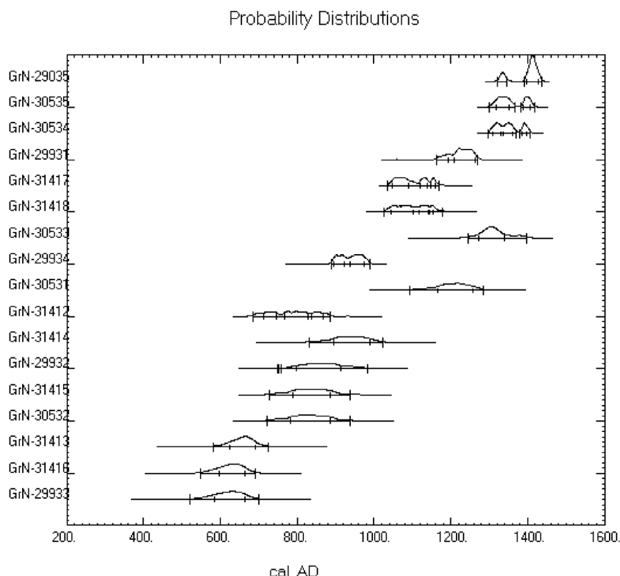
Figure 34. Probability distributions of 14 C dates from El Cabo (CALIB Radiocarbon calibration programme, Stuiver and Reimer 1986-2005).
