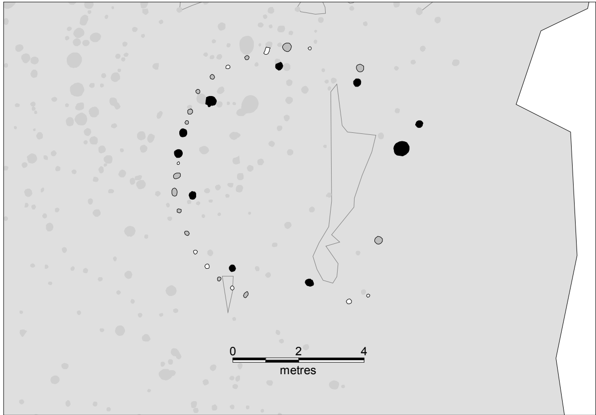
Figure 91. Structure 9.
