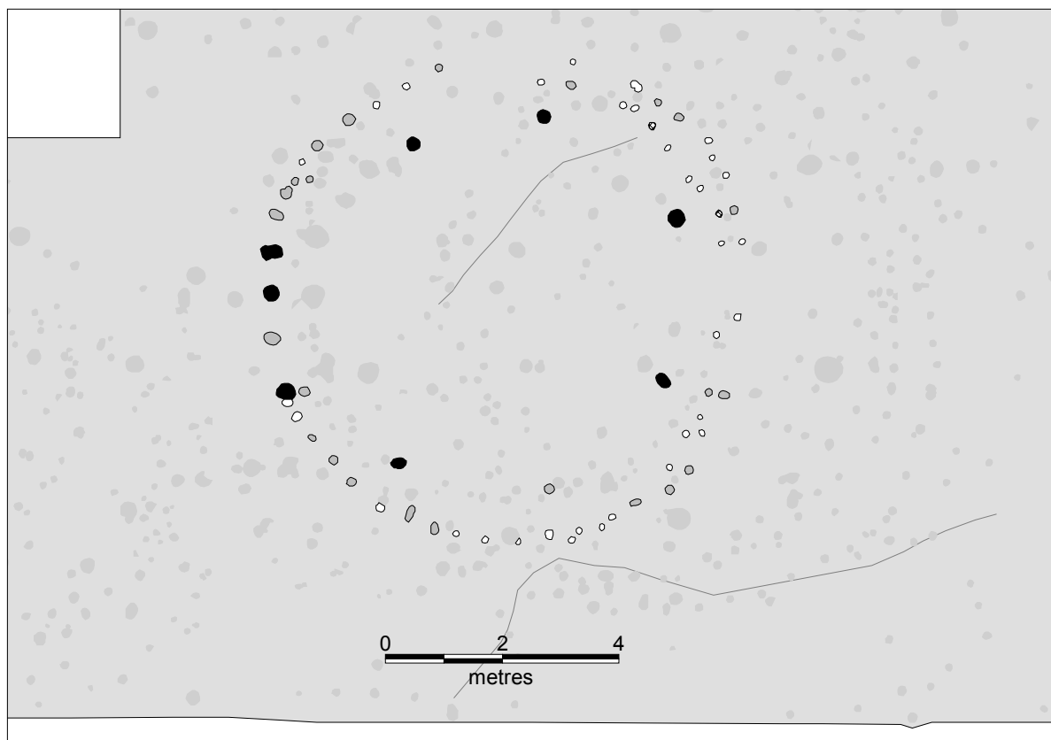
Figure 96. Structure 14.
