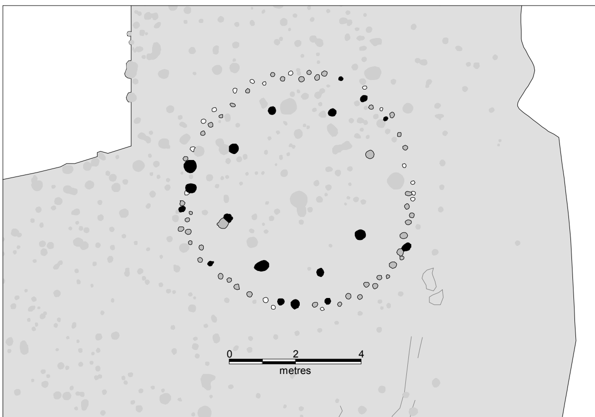
Figure 85. Structure 3.
