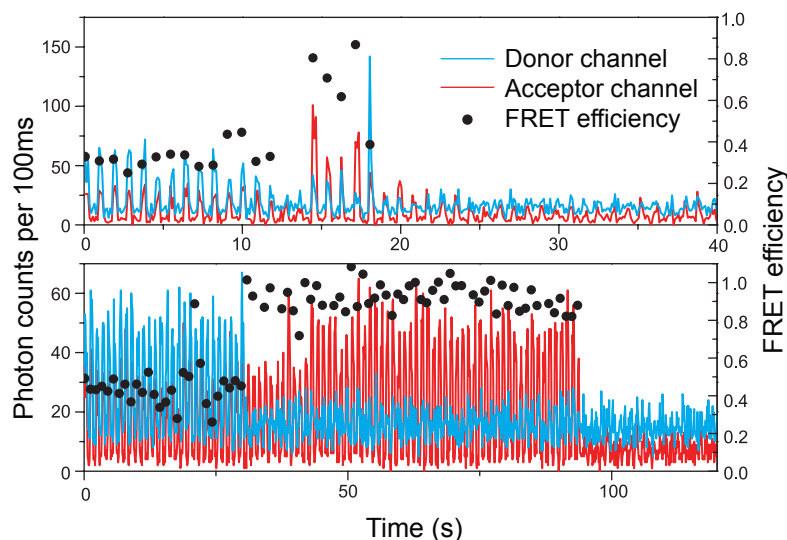
Figure 2.9: Raw temperature-cycle time traces of polyprolin-6 on two different molecules. The light blue and red traces represent the fluorescence signals from the donor and the acceptor respectively; and the black dots are the calculated FRET efficiencies. The peaks of the traces are recorded during the excitation and the lower levels are dark counts from the APDs during the delay time and heating time.
