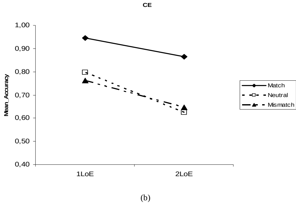
Figure 4. (a) Mean accuracy for 1-, and 2-LoE RB over three semantic types. (b) Mean accuracy for 1-, and 2-LoE CE over three semantic types.
