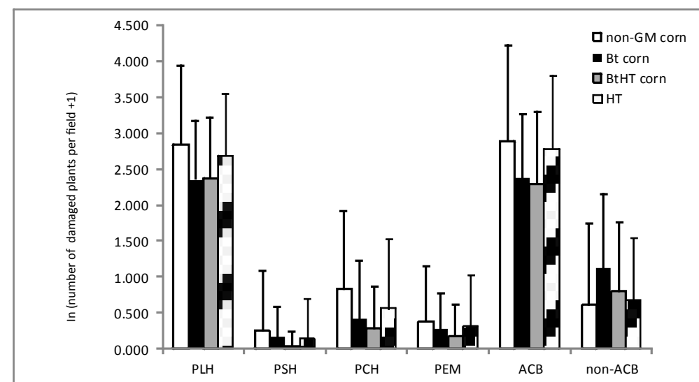
Figure 6. Numbers of damaged plants per field due to ACB and non-ACB pests, for different parts of corn plants (i.e. numbers of holes in leaves, stems or cobs, or number of egg masses). P-values: *** = P < 0.001 , ** = P < 0.01 , * = P < 0.05 , (*) = P < 0.10 .
