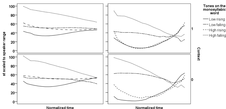
Figure 5.11: Averaged and time-normalized F_0 contours of the four investigated tones in initial (left) and final (right) position, broken down across contexts.
