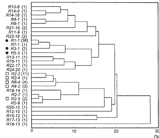
Fig. 3. Cluster analysis of Hind III/ Hinc II ribotypes found in 85 Czech A. baumannii strains. No. of strains with a respective ribotype is indicated in parentheses. Grouping was obtained by the UPGMA algorithm by using percentage disagreement. ●, Ribotypes of strains of AFLP cluster I (clone I); □, ribotypes of strains of AFLP cluster II (clone II).
