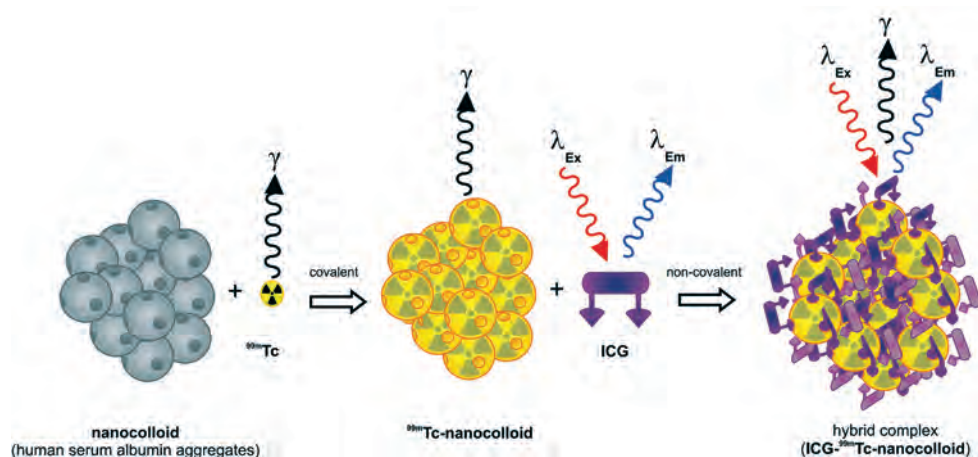
Scheme 1. Schematic representation of the subsequent albumin colloid radiolabeling with ^{99m}\text{Tc} and fluorescent labeling with ICG.
