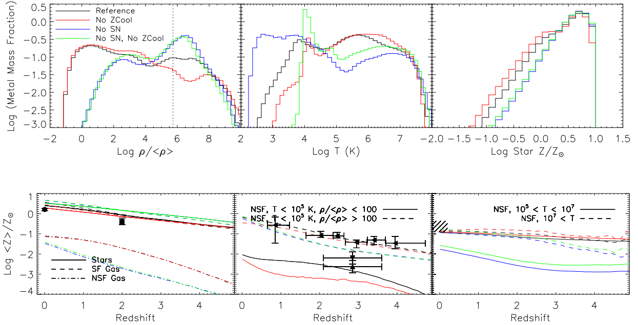
Figure 4.8: Distribution of metals for L100N512 simulations with different feedback and cooling prescriptions. Top panels: z = 0 metal mass weighted PDFs of density, temperature, and stellar metallicity. In the left-most panel, the star formation threshold is indicated by the dotted line. The gas that is on our equation of state was removed from the temperature PDF. Bottom panels : Metallicity as a function of redshift for various phases as defined in figure 4.1. The left panel shows stars (solid), SF gas (dashed) and NSF gas (dot-dashed). The middle panel shows cold IGM (NSF, \rho < 10^2 \langle \rho \rangle , T < 10^5 \text{ K} ; solid), and cold halo and circum-halo gas (NSF, \rho > 10^2 \langle \rho \rangle , T < 10^5 \text{ K} ; dashed). Finally, the right panel shows WHIM (NSF gas, 10^5 \text{ K} < T < 10^7 \text{ K} ; solid) and ICM (non-star-forming, T > 10^7 \text{ K} ; dashed). Shown are the REFERENCE simulation (black), a simulation which cools only using primordial abundances (NOZCOOL; red), a simulation which has no energy feedback (NOSN; blue), and a simulation which has no energy feedback and cools only using primordial abundances (NOSN_NOZCOOL; green), as indicated in the top left panel. Note that the metallicity of the diffuse IGM for the simulations without feedback is below the range in the bottom-middle panel. Data points indicate observations as in figure 4.4, where the points in the left panel correspond to stellar metallicities, the left pointed triangles in the middle panel correspond to the cold halo gas while the other (lower) set of triangles correspond to diffuse IGM measurements and the hatched region in the right panel shows an ICM metallicity measurement. metal-line cooling and especially feedback clearly play a major role in shaping the metallicity of the diffuse IGM. Without supernova feedback, the metallicities of the WHIM and the diffuse IGM are greatly reduced. The effect of feedback is surprisingly small for the metallicity of hot ( T > 10^7 \text{ K} ) gas, stars, and SF gas.
