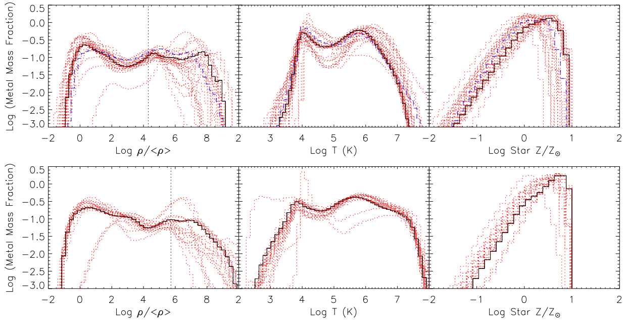
Figure 4.7: Fraction of metals in gas as a function of density (left), temperature (middle) and fraction of metals in stars as a function of stellar metallicity (right) for the same models as shown in figure 4.6 at z = 2 (top) and z = 0 (bottom). Each pdf is normalised to unity. The reference simulations are given in solid black, while the rest of the simulations are shown in dotted red. The REFERENCE_L100N512 model at z = 2 is shown in the top panel with the dashed blue line. SF gas is omitted from the central panel, since the ‘temperature’ of this multi-phase gas is set by the imposed p - \rho relation. The dotted vertical line is the star formation threshold. While there are a few outliers, most models generally yield similar metal distributions, with the biggest differences occurring at high \rho and small T .
