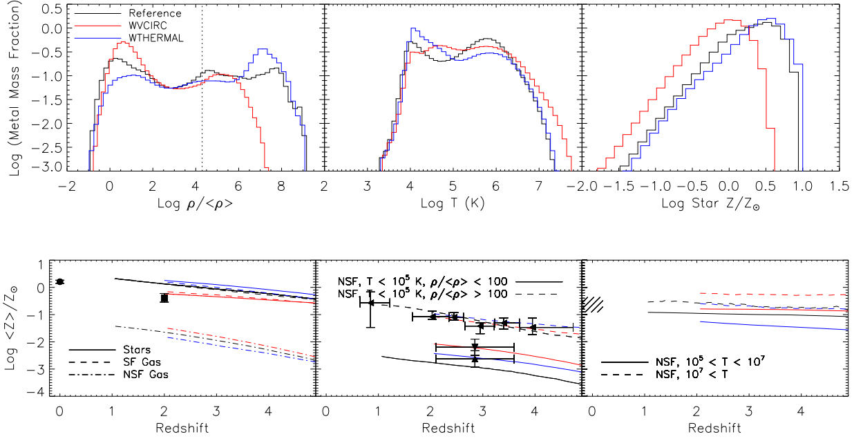
Figure 4.13: As figure 4.8, but for L025N512 simulations, comparing the REFERENCE simulation (black) to model WVCIRC (red), in which wind speed depends on the depth of the potential well (equation 4.6), and model WThermal in which SN energy is injected thermally (blue). The metal mass weighted PDFs are for z = 2 . The WVCIRC model is able to evacuate metals from high density regions, while at the same time, spreading the metals among a variety of temperatures. The WThermal model differs less dramatically from the REFERENCE model, with more metals ending up in high density regions. These three models differ considerably in metallicity evolution in several phases, most notably in the IGM and WHIM; stellar metallicities are lowered in the WVCIRC model.
