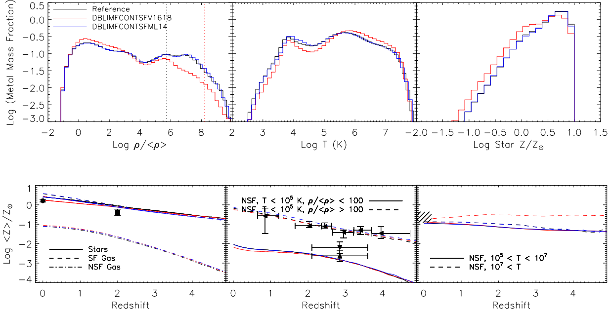
Figure 4.15: As figure 4.8, but for L100N512 simulations comparing the REFERENCE simulation (black), with two models with a top-heavy IMF at high-pressure; one in which the extra wind energy is used to increase the wind velocity ( v_w = 1618 \text{ km s}^{-1} , DBLIMFCONSTSV1618, red), and one in which the extra wind energy is used to increase the mass loading ( \eta = 14 , DBLIMFCONSTFML14, blue). The metal mass weighted PDFs here are for z = 0 . The black dotted line indicates the star formation threshold as before, and the red dotted line indicates the densities above which the top-heavy IMF is used. Using such an IMF has little effect unless the wind energy is used to increase the wind velocity.
