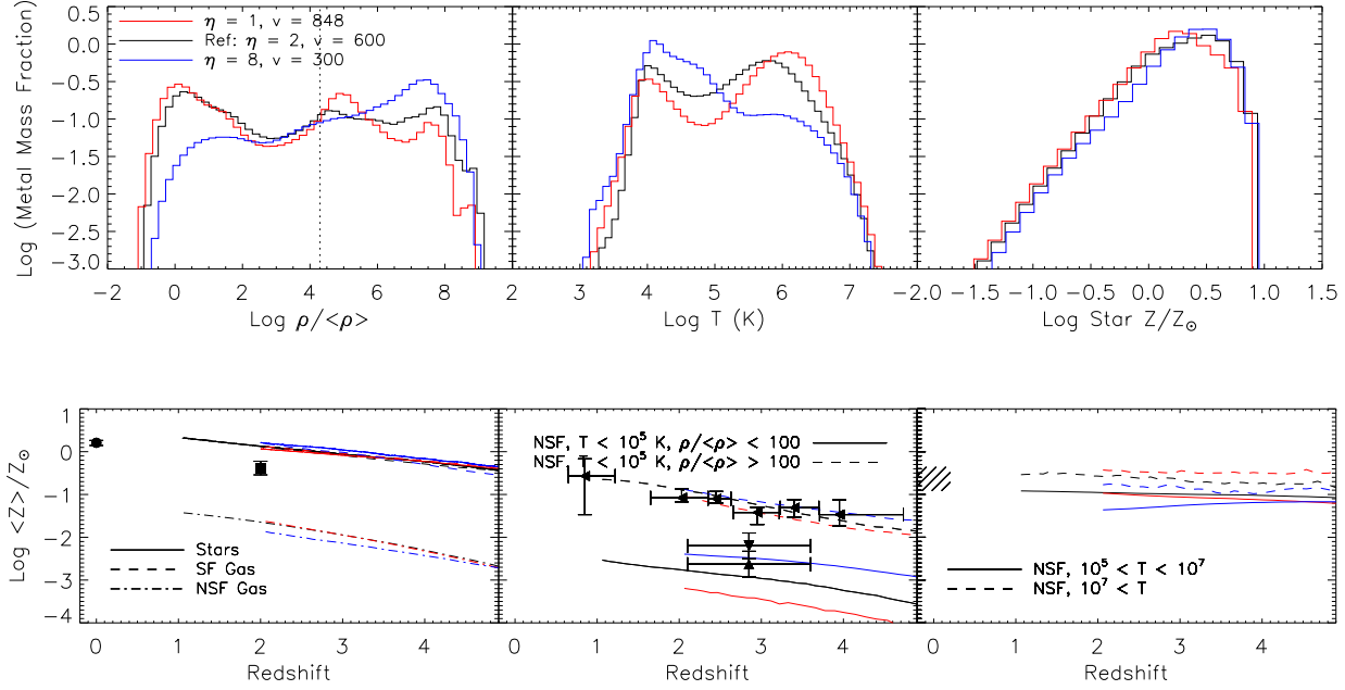
Figure 4.11: As figure 4.8, but for L025N512 simulations with different values for the mass loading, \eta , and wind speed, v_w . The metal mass weighted PDFs (top row) are for z = 2 . Compared are the REFERENCE simulation ( \eta = 2, v_w = 600 \text{ km s}^{-1} ; black), a simulation using a mass-loading of 1 ( \eta = 1, v_w = 848 \text{ km s}^{-1} ; red), and a simulation using a mass-loading of 8 ( \eta = 8, v_w = 300 \text{ km s}^{-1} ; blue). The density and temperature distributions of metals are strongly dependent on \eta . While the choice of \eta has little effect on stellar metallicities, or those of SF gas, the metallicity of the IGM is significantly affected.
