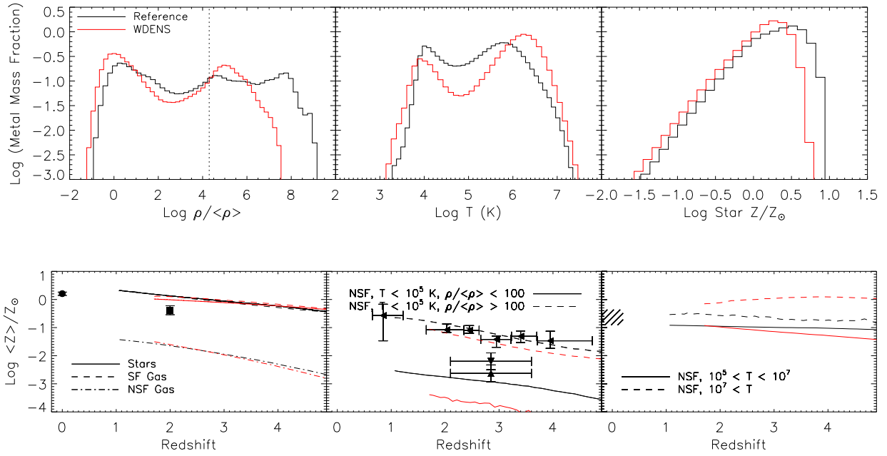
Figure 4.12: As figure 4.8, but for L025N512 simulations comparing the REFERENCE simulation (black) to model WDENS (red) in which wind speed is proportional to the local sound speed (equation 4.5). The metal mass weighted PDFs are for z = 2 . The metallicities of both stars and SF gas are similar between these models, but low density gas is significantly more enriched in the WDENS model; the metallicity of the cold IGM though is lower in the WDENS model. The higher wind speeds in higher mass galaxies allow metals to escape from more massive galaxies in the WDENS models: this raises the ICM metallicity by a factor of a few. The WHIM metallicity is slightly lower initially, but becomes comparable to that of the constant wind model by z \approx 3 .
