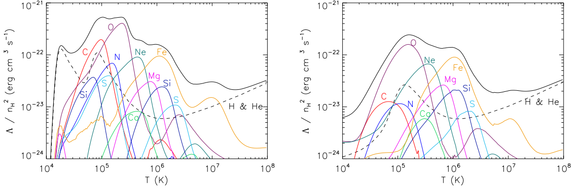
Figure 2.6: Normalized cooling rates as a function of temperature for solar abundances, assuming either CIE ( left-hand panel ) or photo-ionization equilibrium for n_H = 10^{-4} \text{ cm}^{-3} and an optically thin gas exposed to the z = 3 HM01 model for the meta-galactic UV/X-ray background from quasars and galaxies ( right-hand panel ). Note that normalized cooling rates are independent of the density for CIE, but not for photo-ionization equilibrium. The black, solid curve indicates the total cooling rate and the thin, grey, solid curves show the contributions from individual elements. The black, dashed curve shows the contribution from H and He.
