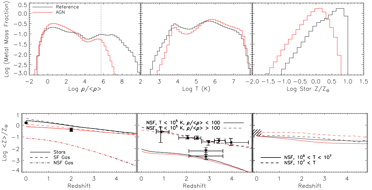
Figure 4.14: As figure 4.8, but for L100N512 simulations comparing the REFERENCE simulation (black) to model AGN (red) which incorporates feedback from AGN. The metal mass weighted PDFs are for z = 0 . The AGN model is also able to evacuate metals from the high-density regions while decreasing the metallicity of stars at z = 0 by \approx 0.5 dex. The metallicities of most of the other phases remains largely unchanged with the exception of the hottest phase whose metallicity increases by a factor of two.
