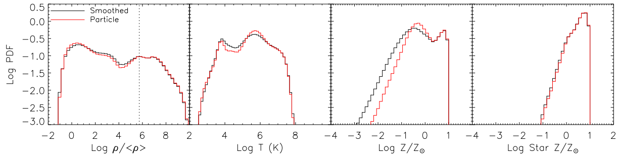
Figure 3.19: Probability density function of the gas density (left), temperature (centre-left) and smoothed/particle metallicity (centre-right) weighted by smoothed (black) and particle (red) metal mass. The black (red) histogram in the right-hand panel shows the PDF of the smoothed (particle) stellar metallicity weighted by smoothed (particle) metal mass. All panels correspond to the L100N512 simulation at z = 0 . The vertical, dotted line in the left panel indicates the threshold for star formation. Note that star-forming gas was excluded from the temperature panel. The predictions for smoothed and particle metallicities only differ significantly for low-metallicity gas.
