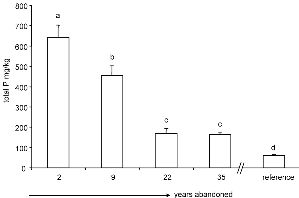
Figure 1: Total phosphorus in the 0-95 cm soil layer of 4 ex-arable fields and a heathland.
