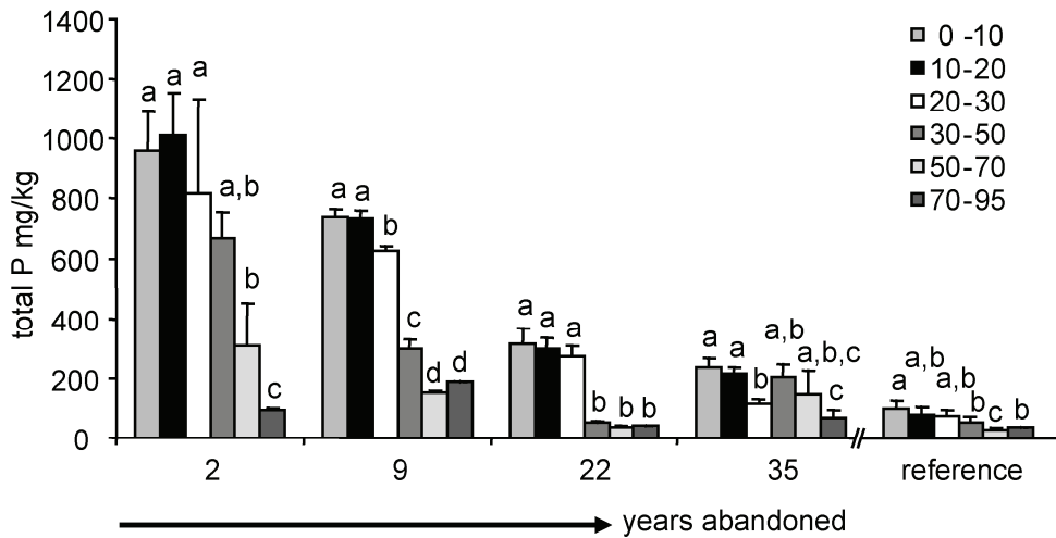
Figure 3: Vertical distribution of total phosphorus in the 0-95 cm layer of 4 ex-arable fields. Given are the total amounts of phosphorus, on basis of dry weight soil, per depth.
