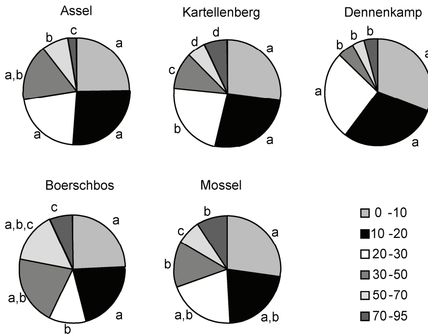
Figure 2: Vertical distribution of total phosphorus in the 0-95 cm layer of 4 ex-arable fields (Assel abandoned since 2 years, Kartellenberg since 9 years, Dennenkamp since 22 years and Boerschbos since 35 years) and a heathland. Given are the percentages of total P, on basis of dry weight soil, per depth.
