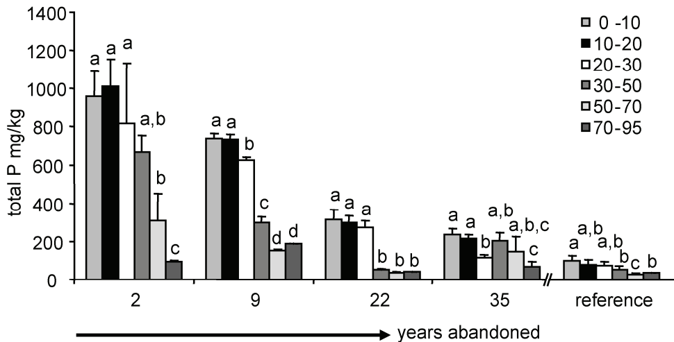
Figure 3: Vertical distribution of total phosphorus in the 0-95 cm layer of 4 ex-arable fields. Given are the total amounts of phosphorus, on basis of dry weight soil, per depth.
