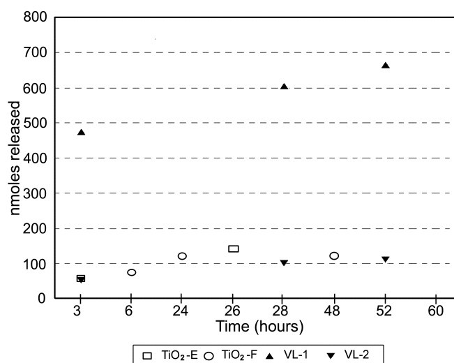
Figure 3. Oxygen release from peroxide-modified titanium dioxide upon humidification compared to the Viking VL-1 Sandy Flats and VL-2 Beta samples.
