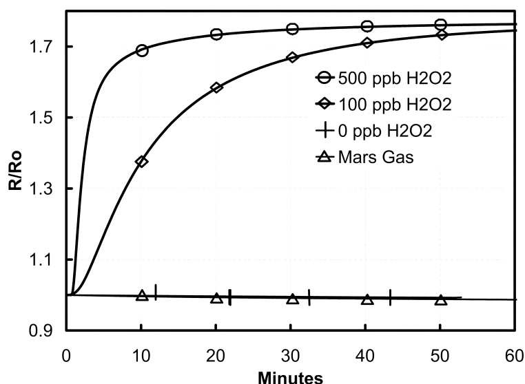
Figure 10.. The sensitivity of freshly deposited films to hydrogen peroxide vapor in carbon dioxide and response of a freshly deposited film to a simulated, peroxide free, martian at-morpheme (0.13% O 2 ; 2.7% N 2 ; balance CO 2 ).
