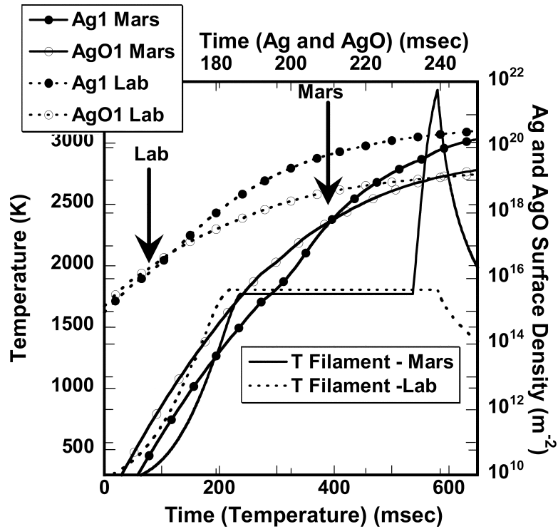
Figure 8. A comparison of the model using the laboratory test conditions with the model using predicted Mars conditions. Both cases, we have adjusted the ambient \text{H}_2\text{O} pressure to 0.71 Pa, the pressure in equilibrium with ice at 210 K. In all cases, the solid lines represent Mars simulations, the dotted lines represent the laboratory simulations. The filled circles represent the number density of metallic Ag ( \text{m}^{-2} ), deposited on the walls of the tube in finite element i=1 , which corresponds to the inboard edge of the Au electrode. The open circles represent the number density of AgO. Number densities are labeled on the right hand ordinate, and the upper abscissa. The arrows labeled “Lab” and “Mars” indicate the time at which metallic Ag begins to be deposited in excess of AgO in element i=1 . On the left hand ordinate, and the lower abscissa, the thermal history of the metal filament is plotted for the laboratory and Mars experiments.
