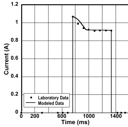
Figure 5. Comparison of the laboratory test data and the modeled sensor behavior. The model correctly predicts the current flow through the circuit. Since \text{heating} = I^2R , the heating rate must likewise be accurate.
