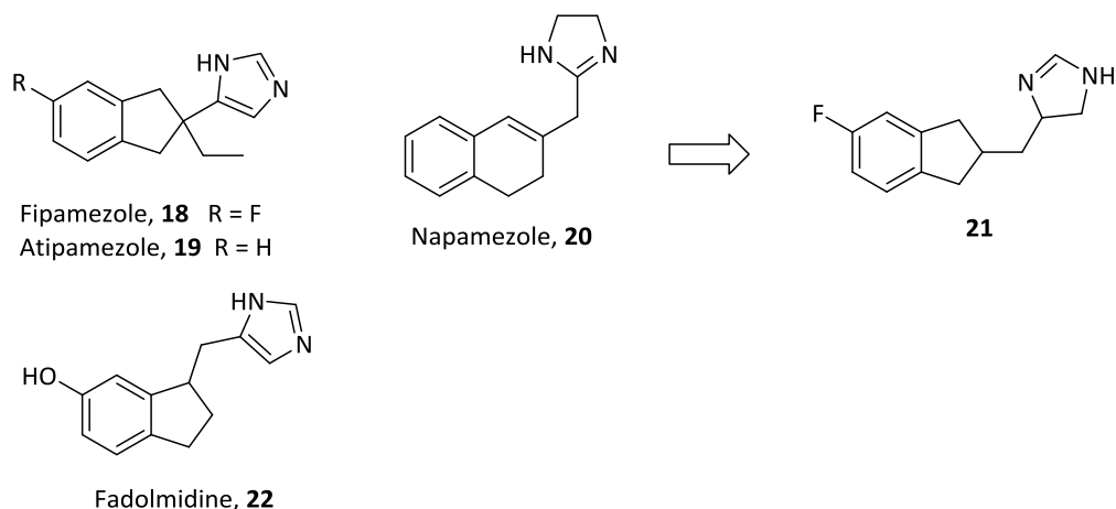
Figure 5. \alpha_2 adrenoceptor ligands.
