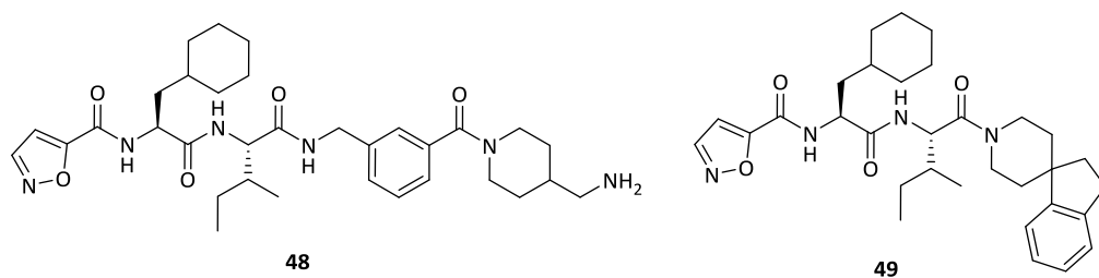
Figure 13. Protease-activated receptor 2 ligands.
