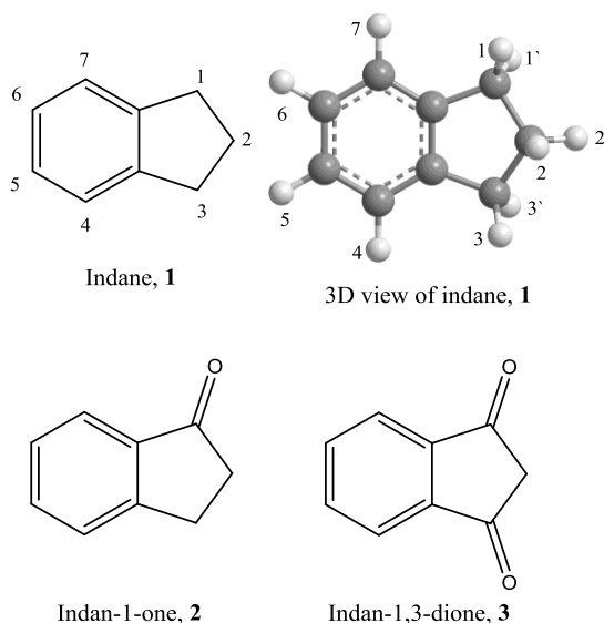
Figure 1. Chemical structures of indane ring system 1 , indan-1-one 2 , indan-1,3-dione 3 .
