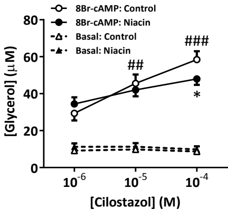
Figure 3: PDE3B capacity of isolated adipocytes after lipolysis stimulation and inhibition. Glycerol concentration in ex vivo gonadal adipocyte medium after 2 h incubation with PDE3B inhibitor cilostazol. A) Responsiveness of basal and 8Br-cAMP stimulated lipolysis to PDE3B inhibition by different cilostazol concentrations. B) PDE3B capacity as glycerol release after PDE3B activation by 10^{-10} M Insulin compared to PDE3B inhibition by 10^{-4} M cilostazol ( \Delta = 8Br-cAMP+Ins+Cilo - 8Br-cAMP+Ins) tested in ex vivo adipocytes from control and niacin treated mice. All values are means \pm SEM. N=10 mice per group, * p\leq 0.05 , ** p\leq 0.01 compared to niacin treatment, ## p\leq 0.01 , ### p\leq 0.001 compared to Cilo 10^{-6} M level.
