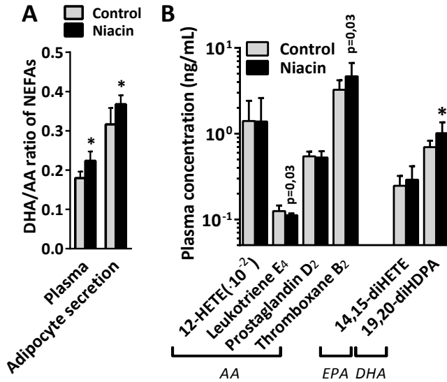
Figure 3: A) Docosahexaenoic acid over arachidonic acid ratio in adipocyte secreted medium and in plasma. B) Oxylipin concentration in plasma of control and niacin treated mice. Mean \pm SD, n=14 per group. * p <0.05 compared to control gWAT after FDR correction. P-values listed were before FDR correction.
