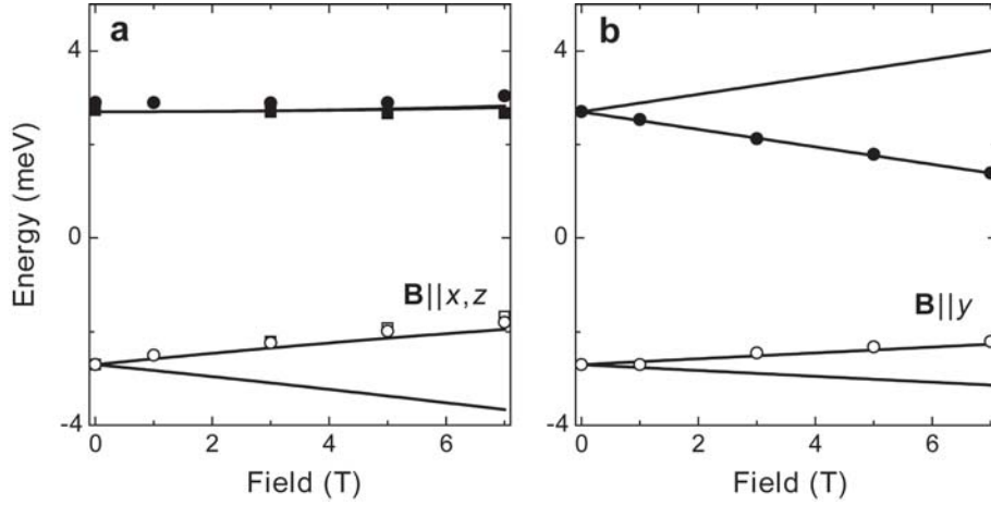
Figure 4.5: Graphs of the peak and step positions taken from fig. 4.4b–d against the field strength for \mathbf{B}||x (circles) and \mathbf{B}||z (squares) in (a) and \mathbf{B}||y in (b). Peak (step) positions are indicated by open (filled) symbols. For the x and z -directions the peak positions are quite similar and therefore hard to distinguish. In contrast to the graphs presented in chapter 3 showing directly the measured excitation energies, here the final energies at the end of the excitation process are plotted: each data point indicates a measured excitation energy added to the calculated ground state energy at the corresponding field. Accordingly, the solid lines show the calculated eigenenergies (rather than the calculated excitation energies as before).
