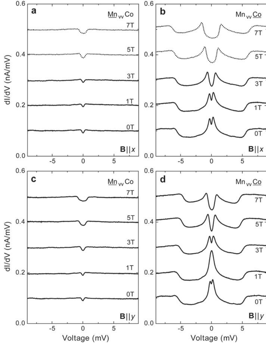
Figure 4.8: dI/dV -spectra measured on Mn_{vv}Co with the tip over the Mn atom (a, c) and Co atom (b, d) at various magnetic fields oriented along x (a, b) and y (c, d). Dotted spectra were taken on a different structure (identical but built elsewhere on the Cu_2N surface) than those with other field strengths in the same direction.
