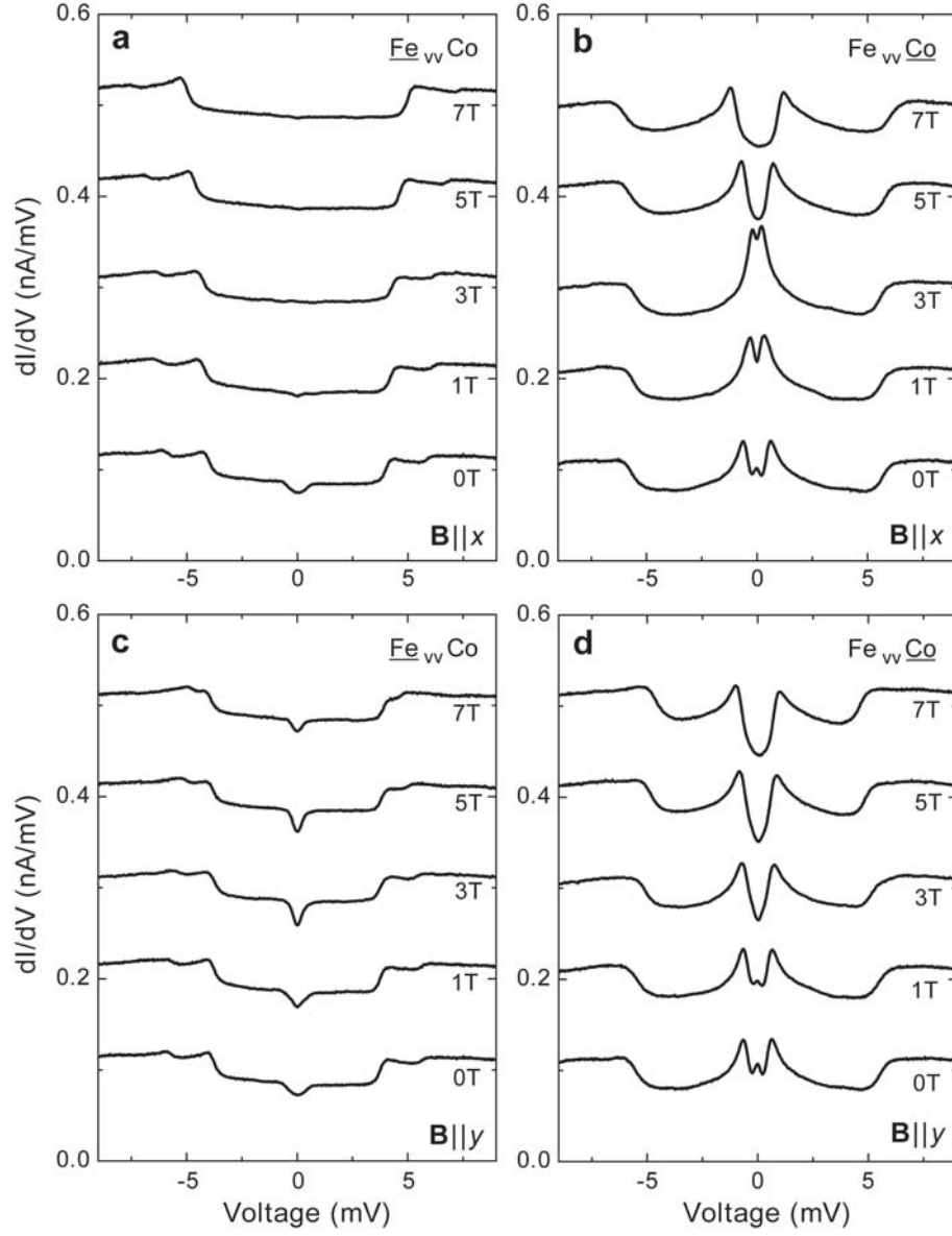
Figure 4.7: dI/dV -spectra measured on \text{Fe}_{\text{vv}}\text{Co} when the tip was positioned over the Fe atom ( a , c ) and Co atom ( b , d ) at various magnetic fields oriented along x (a, b) and y (c, d).
