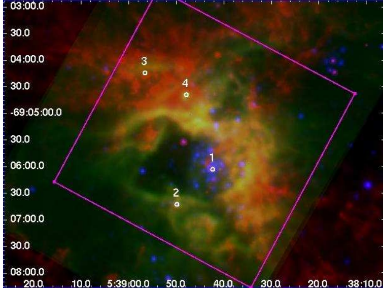
Figure 2.2 Multi-wavelength view of the 30 Doradus region. Red: IRAC 8 \mu\text{m} image showing the PAH emission from the PDR region (c.f. 2.1). Green: [S IV]10.5 \mu\text{m} emission line map, constructed from the spectral map described in §2.2.2, tracing the distribution of highly ionized gas. Blue: Red continuum image showing the stellar continuum emission. White circles mark the positions of the individual spectra discussed in §2.2.3, and their sizes correspond to the size of one resolution element of the spectral map. The magenta square outlines the full IRS spectral map explored in this chapter. North is up and east is to the left.
