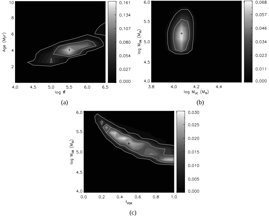
Figure 3.10 Two-dimensional PDFs for selected pairs of parameters covering the totality of the parameter space. The pairs shown are: (a) \log C - t_{cl} , (b) \log M_{emb} - \log M_{cl} and (c) f_{PDR} - \log M_{cl} . The grey scale contours indicate the normalized probability. The cross symbols mark the best-fit values while the white contour lines indicate the 1- \sigma and 90% confidence levels.
