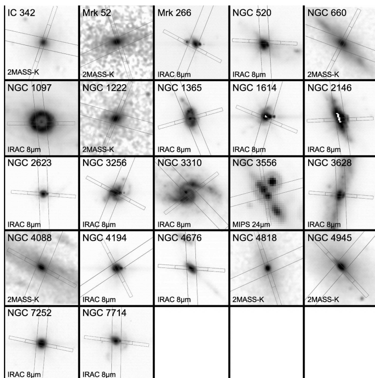
Figure 1.5 Positions of the Spitzer -IRS SL and LL slits overplotted on IRAC 8\,\mu\text{m} , MIPS 24\,\mu\text{m} , or 2MASS K-band images for a sample of starburst galaxies. Figure taken from Brandl et al. (2006).
