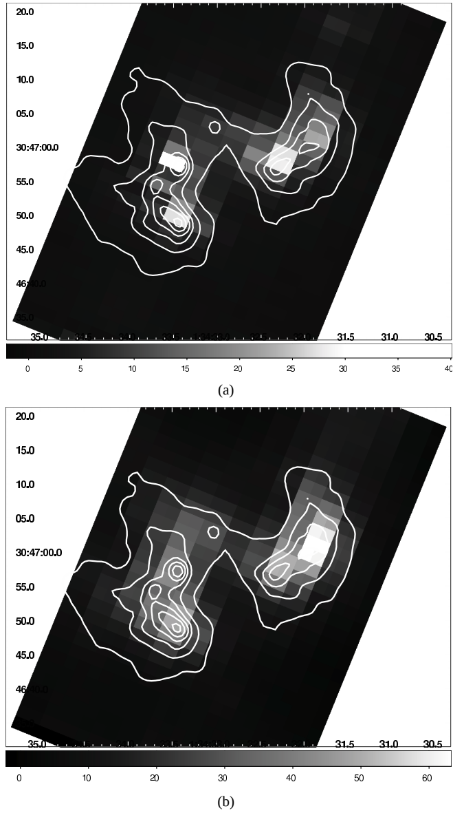
Figure 3.5 Continuum-subtracted line emission in NGC 604, in units of \text{MJy sr}^{-1} . (a) [\text{S IV}]10.5\mu\text{m} emission has well defined peaks near sources 1, 4 and C. (b) [\text{Ne II}] peaks near source 7. The white contours are IRAC 8\mu\text{m} emission.
