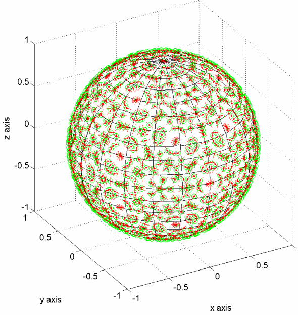
Figure 2. Polar representation of 5880 sampled rotation quaternions using subsampling of the 4D hexacosichoron. Green points represent the viewing directions, whereas the red bars indicate the in plane rotations. The angular distance is about 7.59^\circ .
