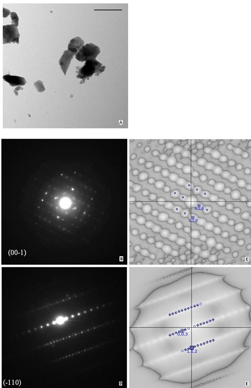
Figure 4 (A) Crystals of potassium penicillin G (scale bar: 2 \mu\text{m} ). (B-E) Electron diffraction patterns and corresponding autocorrelation patterns of potassium penicillin G from two main crystallographic zones. Crosses indicate the centroids of peaks in the
