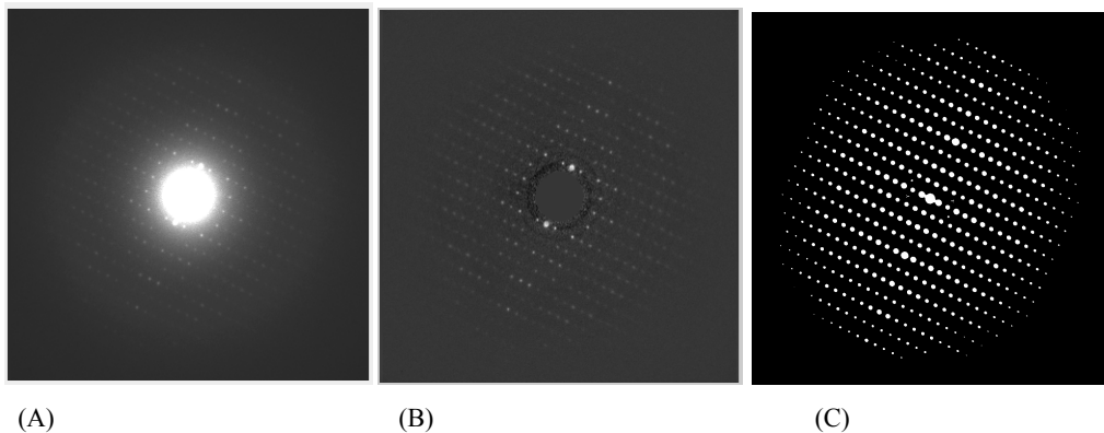
Figure 1 (A) Electron diffraction pattern of lysozyme (electron energy 300 keV). (B) Diffraction pattern after removing the central beam and subtracting the radial background (C) Auto-correlation pattern of B. The diffractogram in Figure 1(A) shows a regular, point symmetrical pattern. The flatness of the Ewald sphere (the wavelength of 300 keV electrons is approximately 0.019 \text{ \AA} ) causes this regularity.
