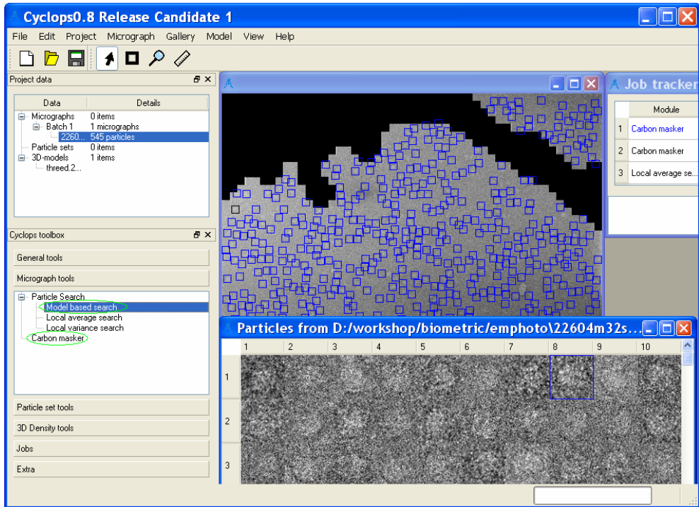
Figure 6. Cyclops has a friendly graphic user interface (GUI) and plug-in architecture. The new algorithms for carbon masking and uniform sampling of rotation space (applied in model based particle searching) are marked by green ellipses. In the sub-window of micrograph, the black area is the result of automated carbon masking, blue boxes indicate selected particles, which are segmented and shown in the sub-window of particles gallery below.
