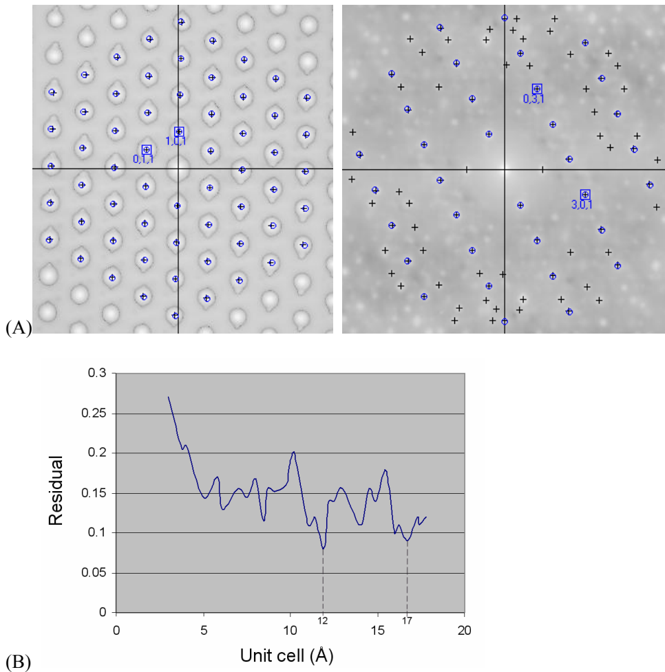
Figure 3 (A) Examples of autocorrelation patterns from experimental electron diffractograms of mayenite. Crosses indicate the centroids of the peaks of the autocorrelation image used for the calculation and circles indicate the peak positions of the simulated diffraction pattern. The extra peaks in the second autocorrelation pattern were caused by low intensity extra lattices in the original diffractogram (not shown). (B) Fine grid search of the unit cell (based on 8 images). The 'Residual' value on the horizontal axis is defined as the square root of the average weighted residual in equation (4).
