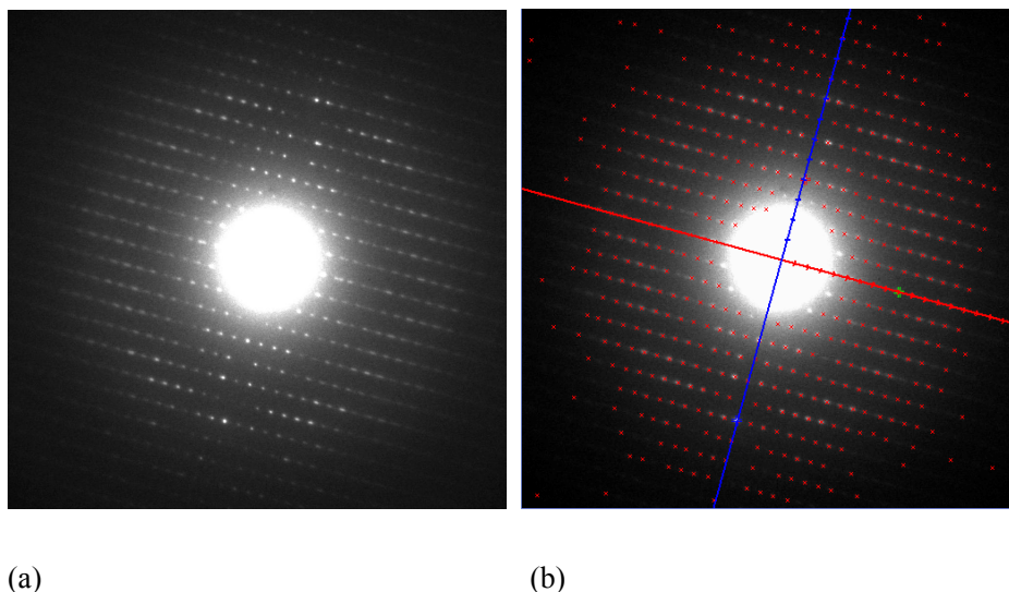
Figure 5 (a) Diffraction pattern from a lysozyme nano-crystal; (b) lattice indexing performed with ELD, using the cell parameters for lysozyme obtained by the algorithm described here. The directions of the shortest reciprocal spacings, given in blue and red and corresponding to the (100) and (011) axes, respectively, are indicated.
