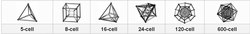
Figure 4. Wireframe perspective projections of six convex regular 4-polytopes. (From wikipedia)
