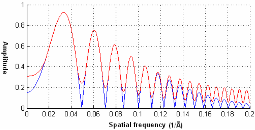
Figure 2. Blue: Theoretical CTF curves after phase flipping. Red: The approximation of the CTF ( =1/G(s) ) used in the inverse filter (after phase flipping)
