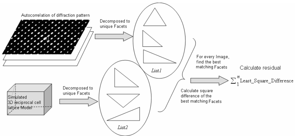
Figure 2 For a given unit cell, a 3D reflection lattice can be calculated. For each characteristic facet from the experimental diffraction pattern, the corresponding facet in the 3D reflection lattice which fits best is identified. The squared distance differences between calculated and experimentally found facets are accumulated in a penalty function.
