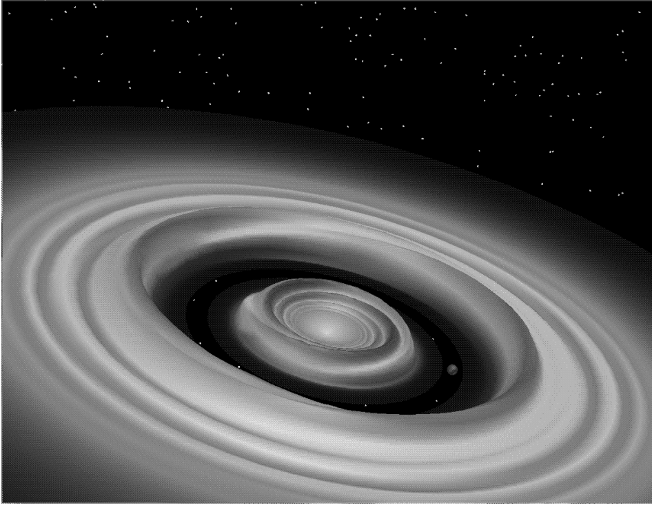
Figure 1.4: Rendering of a hydrodynamical simulation by Bryden et al. (1999) of gap opening in a disk by a giant planet (seen to the right of the central star). The density waves induced by planet-disk interaction are clearly visible.
