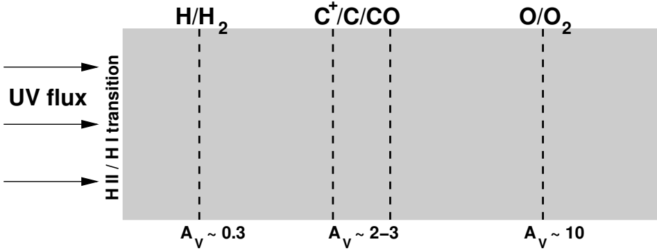
Figure 1.5: Typical structure of a photodissociation region. At the surface all molecules are dissociated by the incident UV flux. With increasing visual extinction, first hydrogen turns to molecular form, followed by carbon (in the form of CO) and oxygen.
