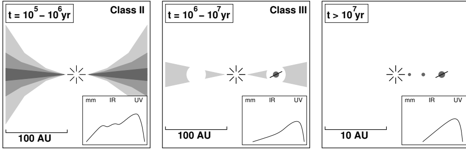
Figure 1.2: As Figure 1.1, but for the final stage of star formation, and the evolution of a circumstellar disk: 4) an optically thick flaring disk, 5) an optically thin debris disk with possible gaps opening due to planet-disk interactions, 6) a main-sequence star that has dispersed its entire disk where only a planetary system is left.
