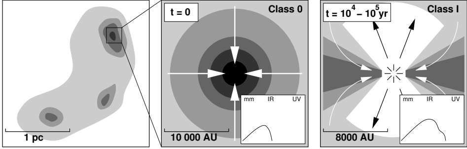
Figure 1.1: Stages 1–3 of low mass star formation according to Shu et al. (1987): 1) slowly contracting dense molecular cores, 2) unstable cores undergoing gravitational collapse, 3) a protostar collecting material via an active accretion disk surrounded by a remnant envelope. Length scales and timescales since the onset of collapse are indicated in the lower left and upper left corners, respectively. The lower right corner shows a typical SED for the object under consideration.
