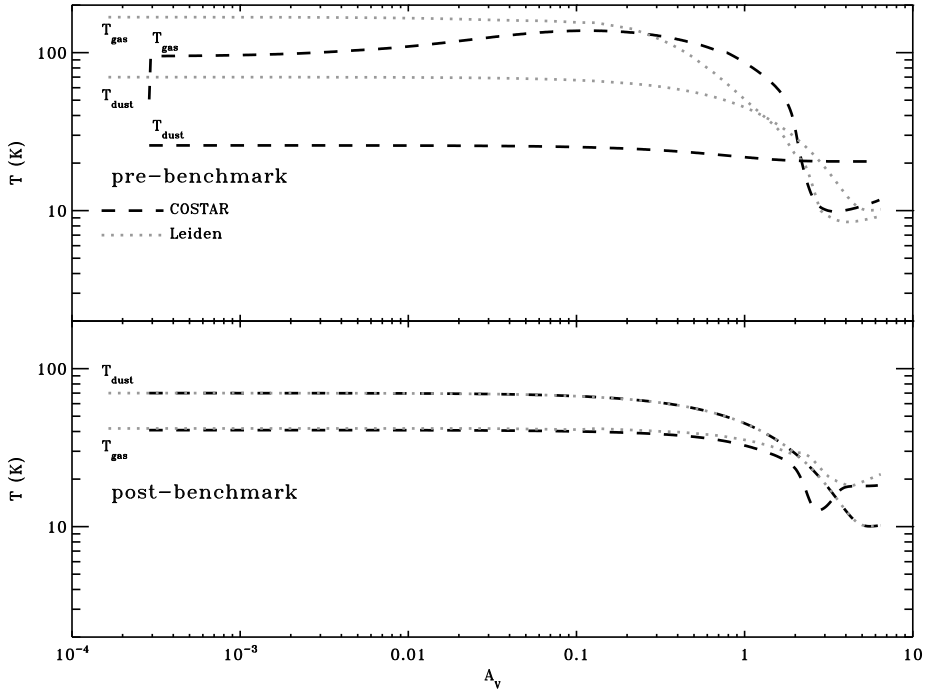
Figure 2.11: The pre-benchmark (top panel) and post-benchmark (lower panel) temperature solutions of COSTAR and Leiden for a separate model to focus on the thermal balance.
