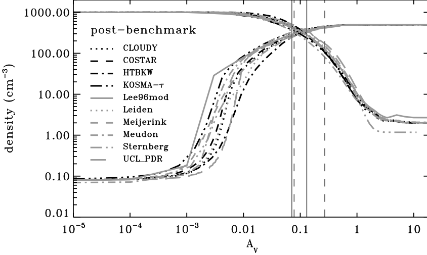
Figure 2.6: Model F1 ( n=10^3 \text{ cm}^{-3} , \chi = 10 ): The H-H 2 transition zone after the comparison study. Plotted is the number density of atomic and molecular hydrogen as a function of A_{V,\text{eff}} . The vertical lines denote the range of the predicted transition depths for pre- and post-benchmark results (dashed and solid lines respectively).
