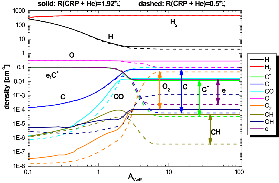
Figure 2.3: Model F1 ( n=10^3 \text{ cm}^{-3} , \chi = 10 ): The influence of the cosmic ray ionization rate on the chemical structure of a model cloud. The solid lines give the results for an ionization rate, enhanced by a factor 4, the dashed lines are for the lower ionization rate. The different greyscales denote different chemical species
