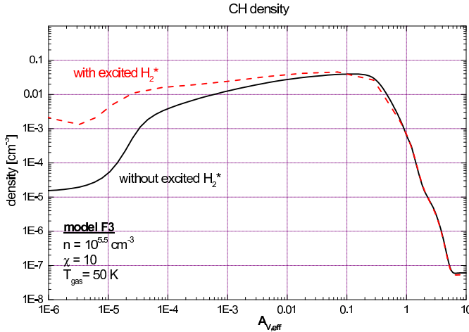
Figure 2.1: Comparison between models codes with (dashed line) and without (solid line) excited molecular hydrogen, H_2^* . The abundance profile of CH is plotted for both models against A_{V,eff} . Benchmark model F3 has a high density ( n = 10^{5.5} \text{ cm}^{-3} ) and low FUV intensity ( \chi = 10 ).
