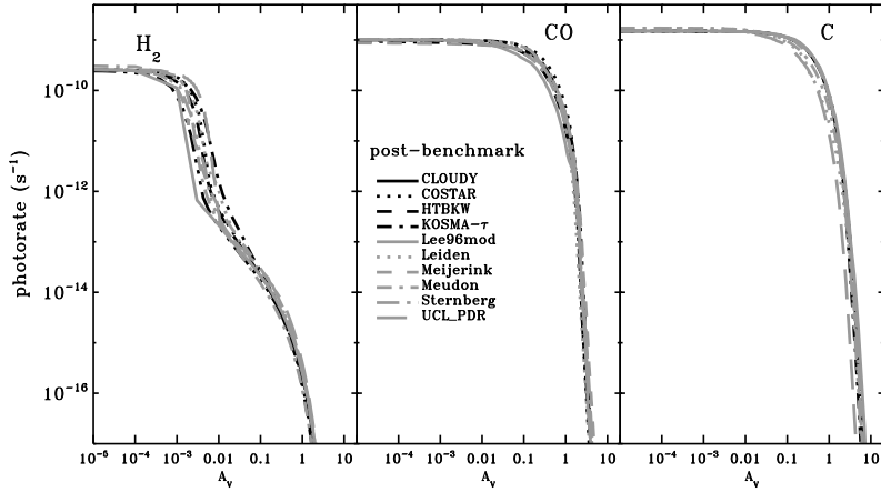
Figure 2.5: Model F1 ( n=10^3 \text{ cm}^{-3} , \chi = 10 ): The photo-dissociation rates of \text{H}_2 (left column), of CO (middle column) and the photo-ionization rate of C (right column) after the comparison study.
