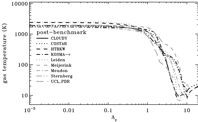
Figure 2.8: Model V2 ( n=10^3 \text{ cm}^{-3} , \chi = 10^5 ): The plot shows the post-benchmark results for the gas temperature.
