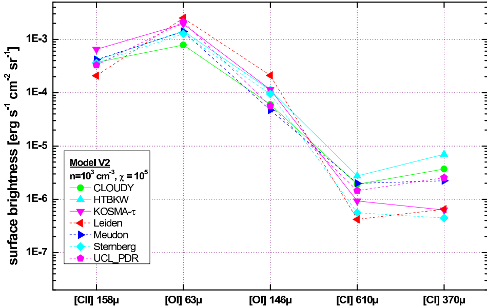
Figure 2.10: Model V2 ( n=10^3 \text{ cm}^{-3} , \chi = 10^5 ): The plot shows the post-benchmark surface brightnesses of the main fine-structure cooling lines: [\text{C II}] 158 \mu\text{m} , [\text{O I}] 63 , and 146 \mu\text{m} , and [\text{C I}] 610 and 370 \mu\text{m} .
