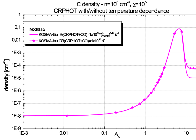
Figure 2.2: The density profile of atomic carbon for the benchmark model F2 (low density, high FUV, as discussed in § 2.5 ). The marked curve results from a constant dissociation by CR induced secondary photons, the unmarked curve shows the influence of a temperature dependent dissociation.
