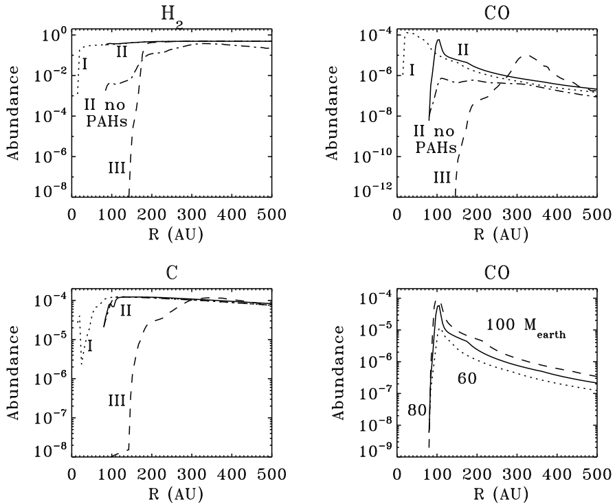
Figure 4.5: Midplane abundances (per H atom) for H_2 (upper left), CO (upper right) and C (lower left) for 80 M_{\oplus} gas distributions I (dotted line), II (solid line) and III (dashed line), and for distribution II when PAHs are removed from the chemistry (dash-dotted line). The lower right panel gives the midplane abundance of CO for gas distribution II with total gas masses of 60 (dotted line), 80 (solid line) and 100 M_{\oplus} (dashed line).
