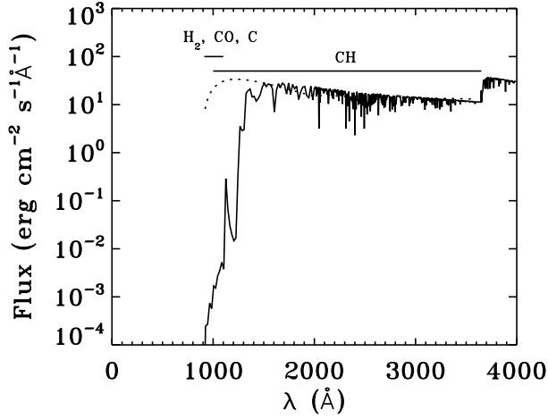
Figure 4.3: The flux at the inner edge of the gas disk in distributions I and III (15 AU from the central star), for the radiation field of a B9.5 star (solid line) and of the interstellar radiation field (dotted line), scaled to fit the integrated flux between 912 and 3600 Å, corresponding to I_{\text{UV}} = 10^7 times the interstellar radiation field. The spectral regime where \text{H}_2 and CO are dissociated and C ionized, and the regime where CH is dissociated are indicated with bars at the top.
