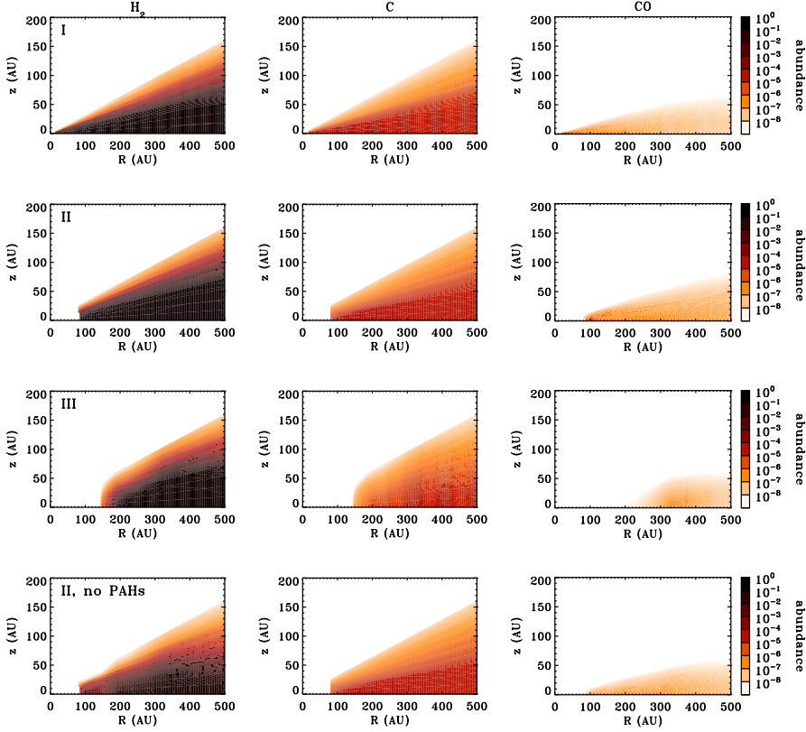
Figure 4.4: Abundances (per H atom) for \text{H}_2 (left column) C (middle column) and CO (right column) for models I (first row), II (second row), III (third row) and II without PAHs (fourth row). In all cases the gas mass is 80 M_{\oplus} .
