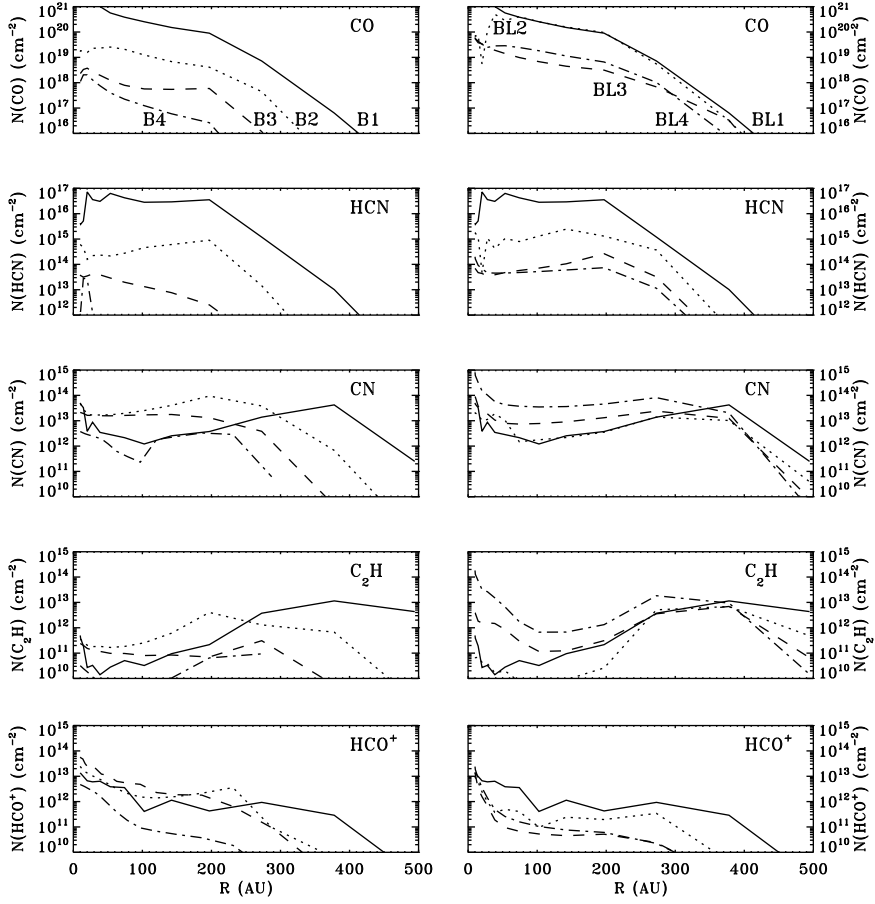
Figure 5.8: The vertical column densities of CO (top row), HCN (second row), CN (third row), C_2H (fourth row) and HCO^+ (bottom row) for the B series (with a descending disk mass, left column) and the BL series (with a descending dust/gas ratio, right column). The solid lines give the results for model B1/BL1; the dotted line for B2/BL2; the dashed line for B3/BL3; the dash-dotted line for B4/BL4.
