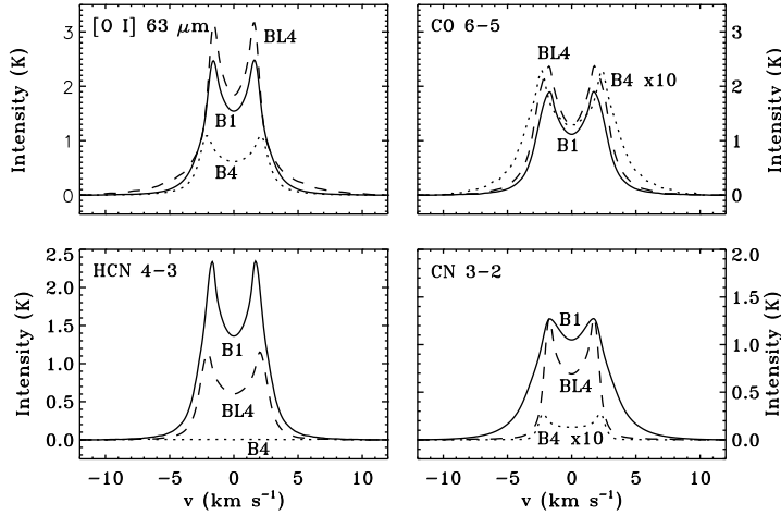
Figure 5.9: Emission line profiles for O (top left), CO (top right), HCN (lower left) and CN (lower right) for models B1/BL1 (solid line), B4 (dotted line) and BL4 (dashed line).
