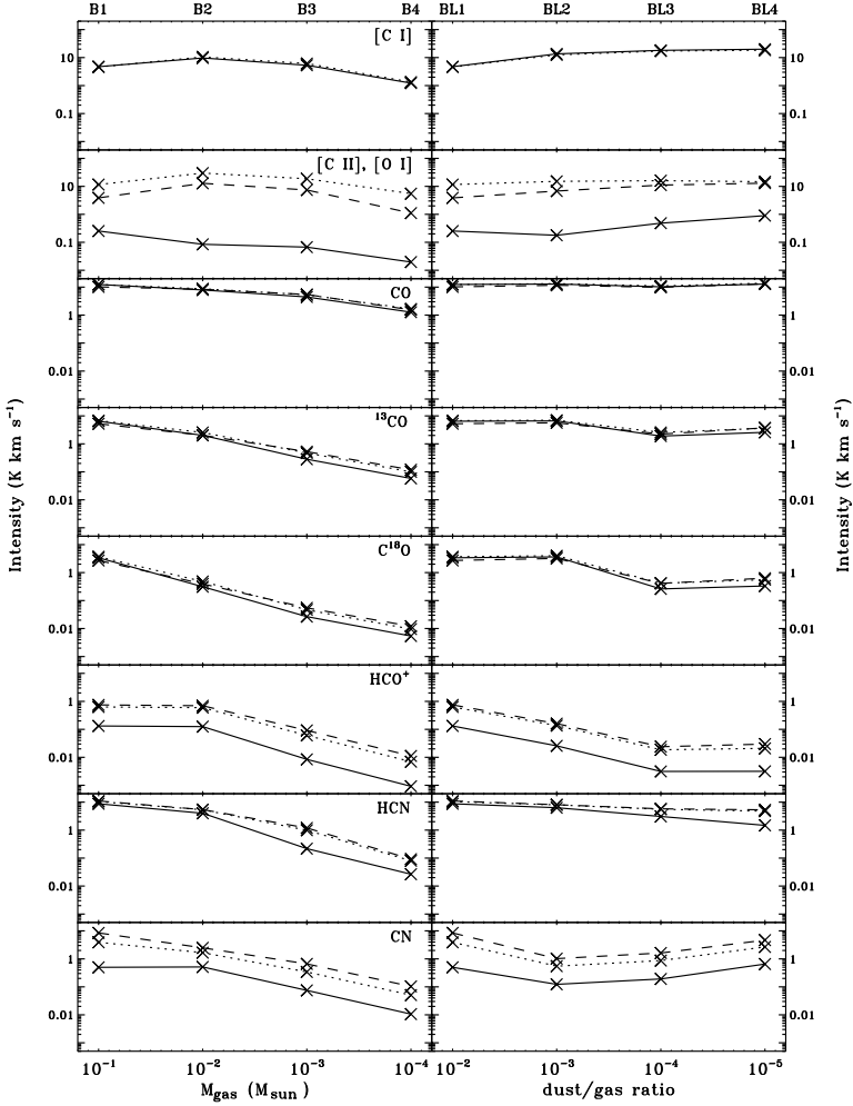
Figure 5.10: Integrated intensities in a 6.7'' beam for the B series (left column) and the BL series (right column). The top row gives the [\text{C I}] fine structure lines ( J = 1 - 0 solid, J = 2 - 1 dotted). The second row gives the fine structure lines of [\text{C II}] fine structure line (solid) and [\text{O I}] ( J = 1 - 2 dotted, J = 0 - 1 dashed). The third, fourth and fifth rows give the rotational lines of \text{CO} , ^{13}\text{CO} and \text{C}^{18}\text{O} ( J = 2 - 1 solid, J = 3 - 2 dotted, J = 6 - 5 dashed). The sixth row gives the rotational lines of \text{HCO}^+ and ( J = 1 - 0 solid, J = 3 - 2 dotted, J = 4 - 3 dashed). The seventh row gives the rotational lines of \text{HCN} ( J = 1 - 0 solid, J = 3 - 2 dotted, J = 4 - 3 dashed). The bottom row gives the rotational lines of \text{CN} ( J = 1 - 0 solid, J = 2 - 1 dotted, J = 3 - 2 dashed).
