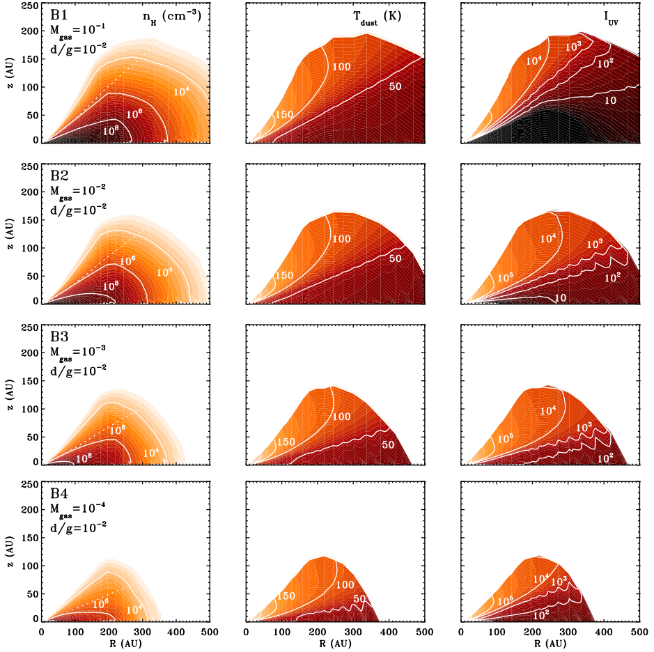
Figure 5.1: Input densities (left column) dust temperatures (middle column) and integrated strength of the UV field (right column) for models B1–B4 of Dullemond & Dominik (2004). The gas mass (in M_{\odot} ) and dust/gas ratio are indicated in the for each row. The UV field is given in terms of I_{\text{UV}} times the strength of the interstellar radiation field by Draine (1978) integrated between 912 and 2050 Å. The dotted lines in the density plots give the boundary where the visual extinction towards the central star is 1 magnitude.
