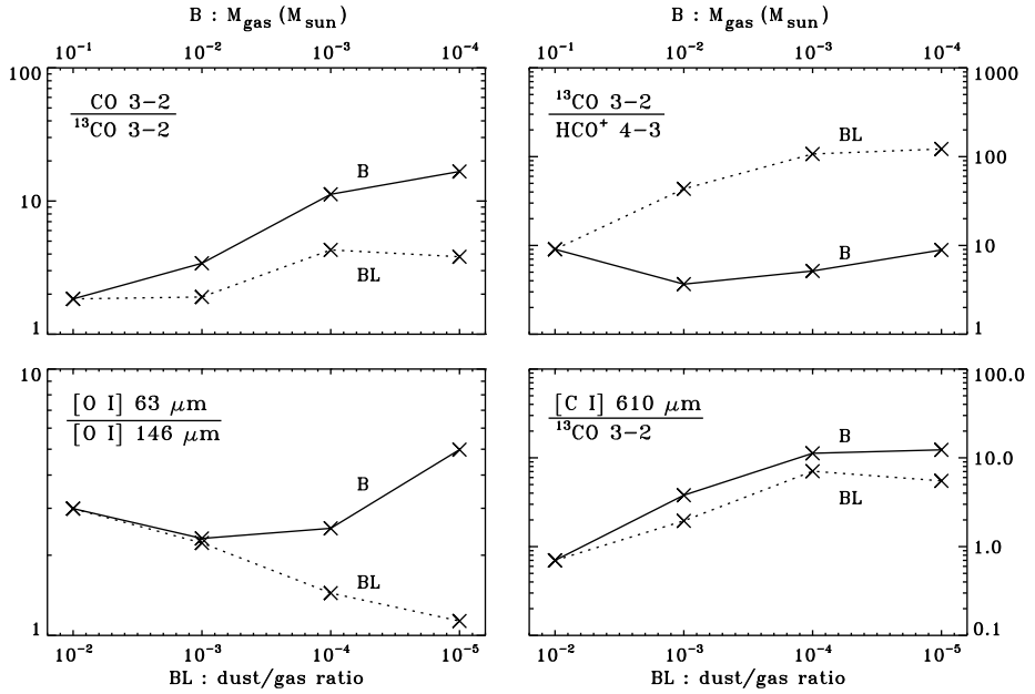
Figure 5.12: Line ratios for the B series (solid lines) and the BL series (dotted lines).
