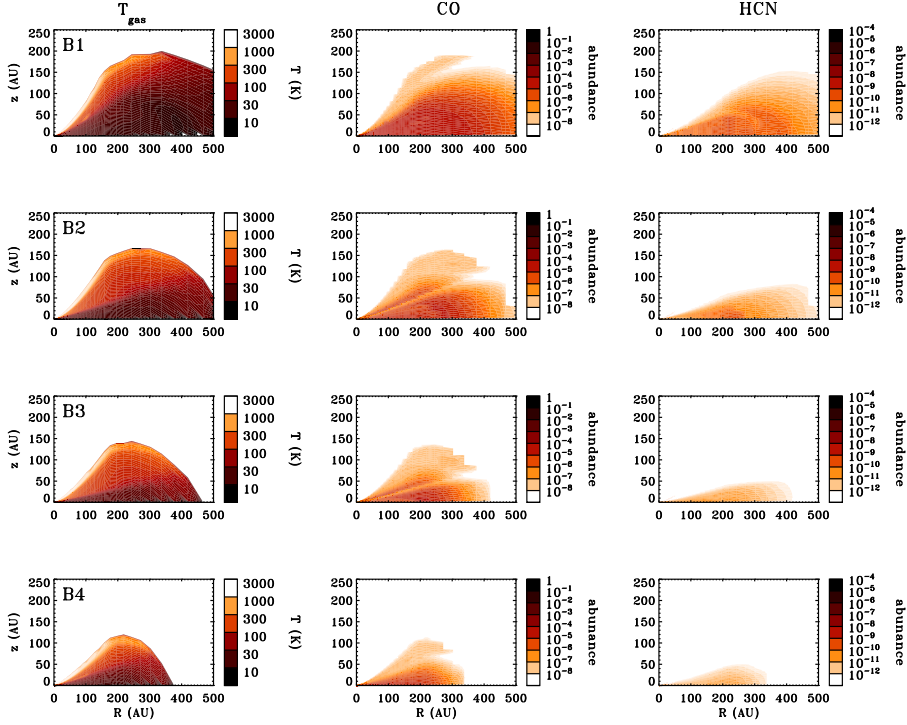
Figure 5.4: Gas temperatures (left column), CO abundances (middle column) and HCN abundances (right column) for models B1–B4.
