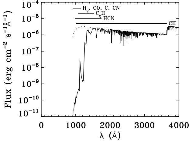
Figure 5.3: The radiation fields used in the model. The solid line gives the stellar radiation field, scaled to the interstellar UV field by Draine (1978) (dotted line). The horizontal lines indicate the wavelength ranges where several important molecules are dissociated.
