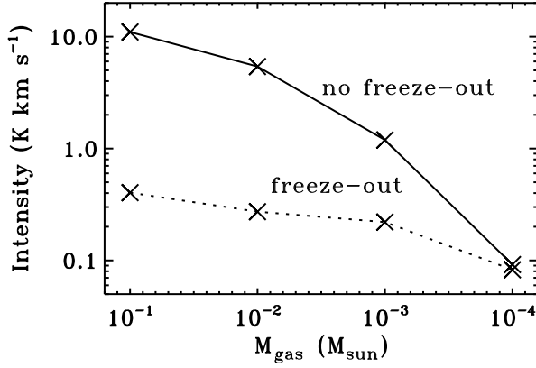
Figure 5.11: Integrated intensities of HCN in the B series when all HCN is in the gas phase (solid line) and when HCN is removed from the gas phase for T_{\text{dust}} < 70 K (dotted line). The BL series follows similar trends.
