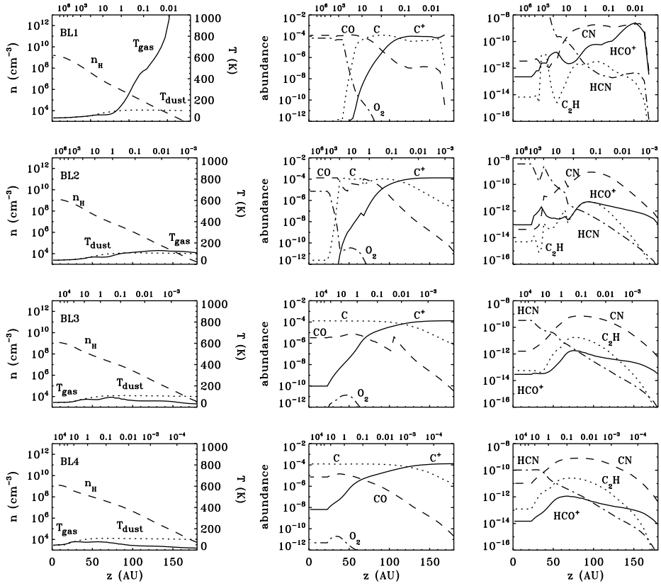
Figure 5.7: As Figure 5.6, but for models BL1–BL4.
