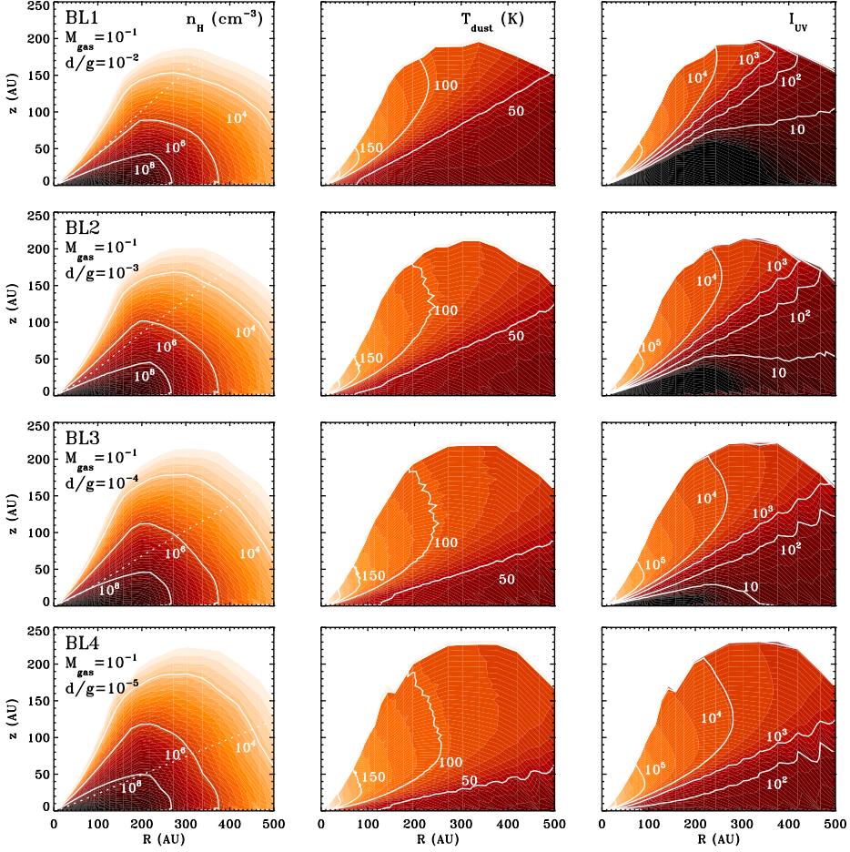
Figure 5.2: As Figure 5.1, but for models BL1–BL4.
