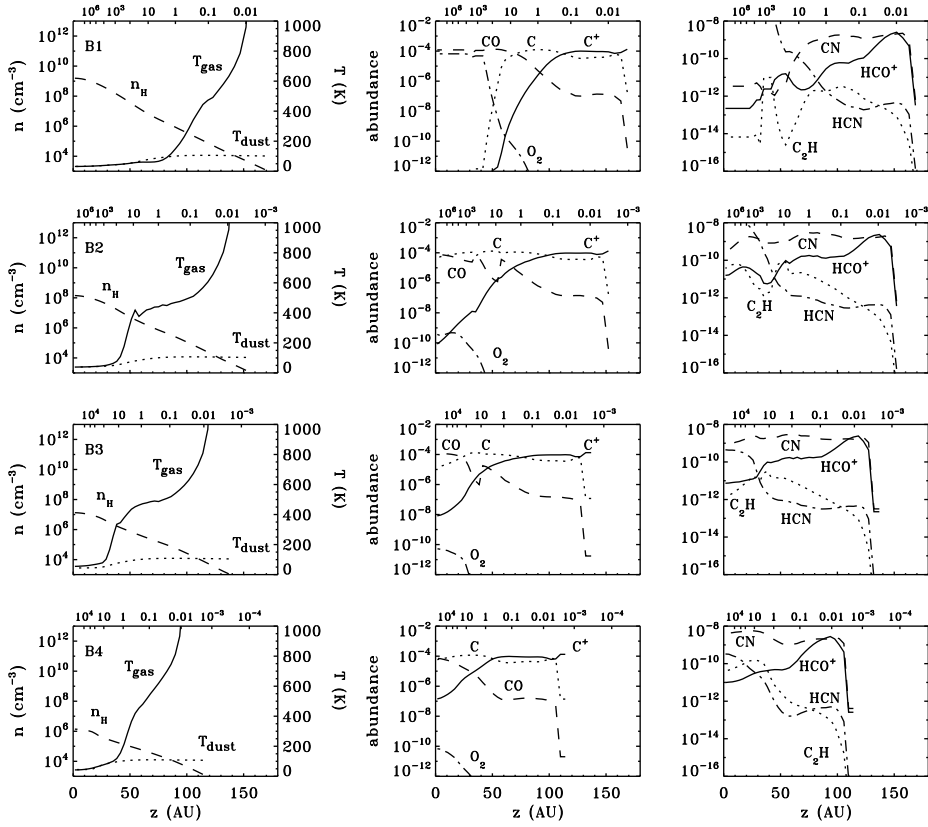
Figure 5.6: Vertical profiles at a radius of 200 AU of the gas temperature and density (left column) and chemistry (middle and right columns) for models B1–B4. The visual extinction toward the central star is given at the top of each panel.
