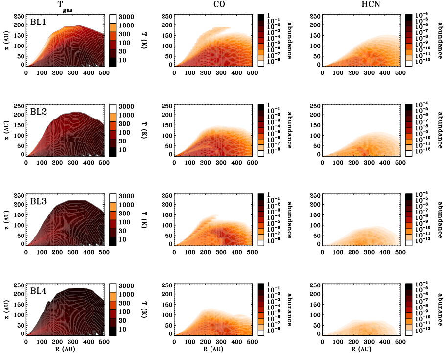
Figure 5.5: Gas temperatures (left column), CO abundances (middle column) and HCN abundances (right column) for models BL1–BL4.
