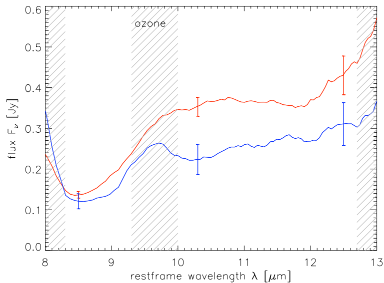
Figure 4.2 — Smoothed ( \Delta\lambda \sim 0.3\mu\text{m} ) correlated MIDI spectra at two different East-West projected baselines: 61\text{m} (red) and 89\text{m} (blue). The errors were taken as the standard deviations from multiple observations. The region of atmospheric ozone absorption, between 9.3 and 10 \mu\text{m} (hatched), is uncertain and not taken into account for the later analysis, as are the regions \lambda < 8.3\mu\text{m} and \lambda > 12.7\mu\text{m} (hatched), which have very low S/N.
