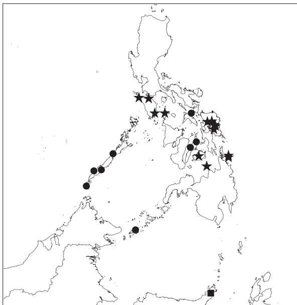
Map 6.3. Distribution of Cleidion microcarpum Merr. (●), C. ramosii (Merr.) Merr. (★) and C. minahassae Pax & K. Hoffm. (■).
