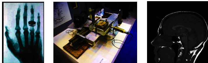
Figure 1.2: From left to right: The first X-ray image, taken by Roentgen in 1896; The first CT scanner prototype designed by Hounsfield; Sagittal MR image of the brain.
