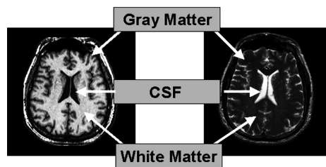
Figure 1.6: MR T1-weighted (left) and T2-weighted (right) axial views of the brain. In T1w images, gray matter is in gray, white matter in white, and CSF in black. In T2w images, the colors are inverted.
