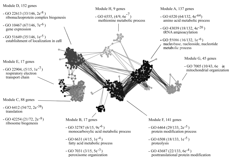
Fig. 5. Assignment of biological functions to modules. For the combined data sets network at a p threshold of 0.90 (as shown in Fig. 3, panel D), enriched biological processes are indicated within modules using the Gene Ontology terms of genes with a S. cerevisiae ortholog. The number of A. niger genes per module is indicated after the module code. The GO-number points to the observed Gene Ontology process. Between brackets, the number of genes with that annotated Gene Ontology process relative to the total number of genes queried is given, followed by a p -value that gives the likelihood that the identified GO process is found by chance alone. Genes that encode conserved proteins but have no S. cerevisiae ortholog make up the difference in the total number of A. niger genes per module and the number of genes queried for Gene Ontology enrichment.
