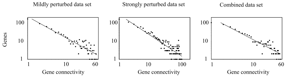
Fig. 4. Gene connectivity distribution per data set. For each gene within the networks at a \rho threshold of 0.90, the number of genes it partners with (horizontal axis) is plotted against the number of genes with identical number of gene pairs (vertical axis). The fitted line is for a power-law distribution, P(k) \sim k^{-\gamma} , which describes the probability that a gene has k gene pairs. For all networks, \gamma is around 1.2.
