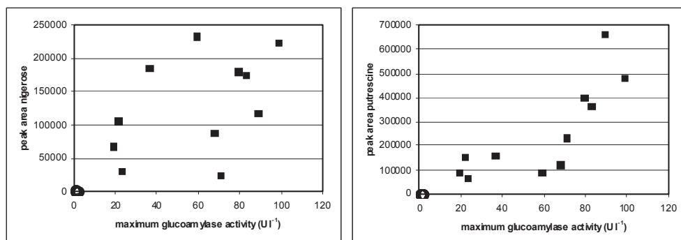
Fig. 3. Plot of the correlation between the metabolite tentatively identified as nigerose and maximum glucoamylase activity (A) and a similar plot for putrescine (B). O, Metabolome samples from xylose fermentations (n=11); ■, metabolome samples from glucose fermentations (n=11).
