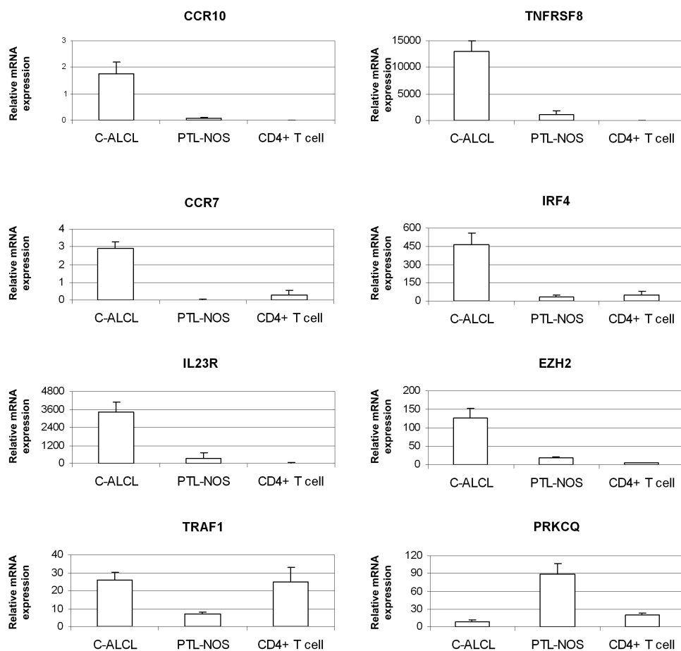
Figure 3 Expression levels of selected genes as measured by qPCR
