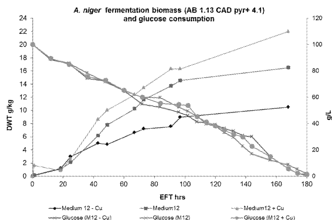
Figure 4. Biomass growth and glucose consumption of A. niger in fermentations with varying copper concentrations. Biomass determination of mycelium in batch fermentation (◆—Medium12-Cu with 0.005 mM \text{Cu}^{2+} ; ■—Medium12 with 0.01 mM \text{Cu}^{2+} ; ▲—Medium12 + Cu with 0.02 mM \text{Cu}^{2+} ). The glucose consumption of three batch fermentations were shown on the secondary Axis (X— Medium12-Cu with 0.005 mM \text{Cu}^{2+} ; □— Medium12 with 0.01 mM \text{Cu}^{2+} ; ●—Medium12+Cu with 0.02 mM \text{Cu}^{2+} )
