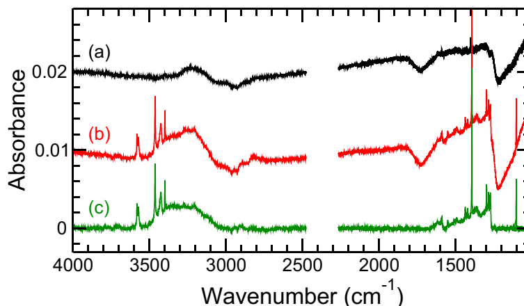
Figure 5.1 RAIR spectra of co-deposited \text{O}_2 and \text{H}_2 without baseline subtraction (a), co-deposited \text{O}_2 and \text{H} without baseline subtraction (b), and co-deposited \text{O}_2 and \text{H} with baseline subtraction (c). \text{H}/\text{O}_2 or \text{H}_2/\text{O}_2 is 2 and the surface temperature is 20 K. The spectra (b) and (c) are displaced on the vertical axis by 0.01 and 0.02, respectively.
