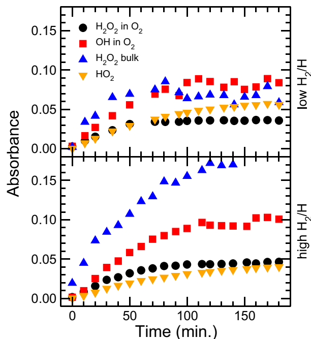
Figure 5.7 RAIRS integrated intensities for \text{H}/\text{O}_2 = 1 and at 20 K with two different \text{H}/\text{H}_2 ratios. The standard, low, \text{H}_2/\text{H} ratio results are plotted in the upper panel; the high \text{H}_2/\text{H} ratio results in the lower panel.
