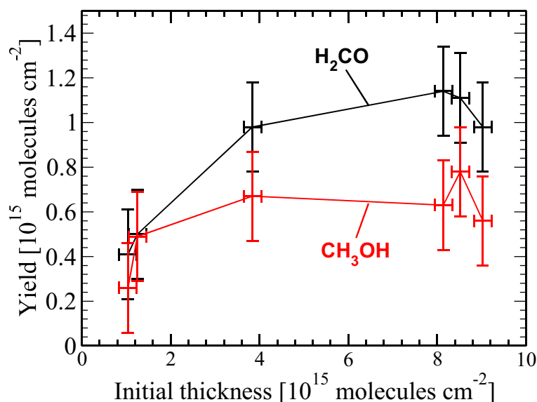
Figure 2.9 The absolute reaction yield of \text{H}_2\text{CO} and \text{CH}_3\text{OH} after a fluence of 5.4 \times 10^{17} \text{H} atoms \text{cm}^{-2} as a function of the layer thickness for experiments at 12.0 K.
