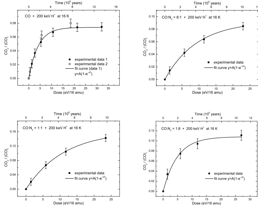
Figure 9.2 Column density of \text{CO}_2 divided by the initial column density of \text{CO} before irradiation for pure \text{CO} ice and \text{CO}:\text{N}_2 mixtures. The column density ratio is plotted as a function of dose. The dose is transferred to interstellar timescales as indicated on the top x -axis. Experimental data are fitted to an exponential curve (Eq. (9.1)): y = A[1 - e^{-(\sigma D)}] , where A is the asymptotic value for \text{CO}_2 column density divided by the initial column density of \text{CO} , \sigma is the total cross section, and D is the dose. Only the points indicated by data 1 (990 nm thick sample) are used for the fit in the top-left panel. Data 2 (220 nm thick sample) is plotted for comparison.
