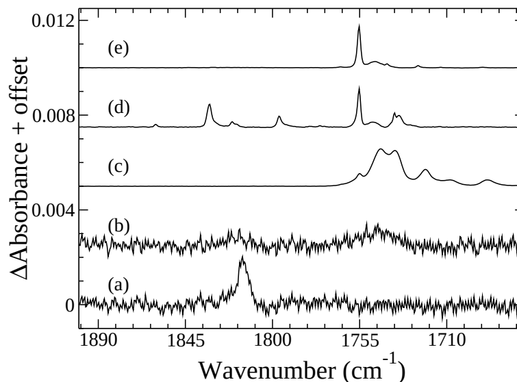
Figure 8.3 Infrared spectra from a H-atom and \text{CO}:\text{O}_2 = 4:1 co-deposition experiment at 15 K (a), and 30 K (b) compared to a spectrum of \text{CO}:\text{HCOOH} = 100:1 at 15 K (c), a spectrum from a \text{CO}:\text{O}_2 = 100:1 co-deposition experiment at 15 K (d), and a spectrum of \text{CO}:\text{HCOOH} = 1000:1 at 15 K (e) using higher H-atom flux ( 2 \times 10^{14} \text{ cm}^{-2} \text{ s}^{-1} ) and \text{CO}:\text{O}_2 flow ( 1 \times 10^{14} \text{ cm}^{-2} \text{ s}^{-1} ). Spectra are offset for clarity.
