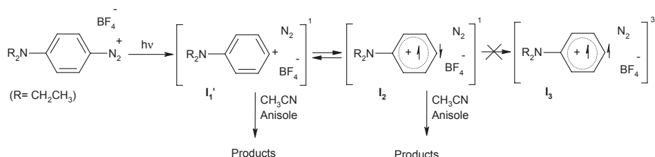
Scheme 6: Mechanism of the photolysis of 4-diethylaminophenyldiazonium salt 6 .
