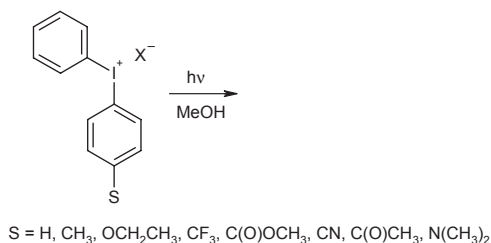
Scheme 8: Photochemical reactions studied in Chapter 2.
