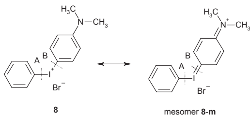
Scheme 4: Mesomeric structure of 8 .
