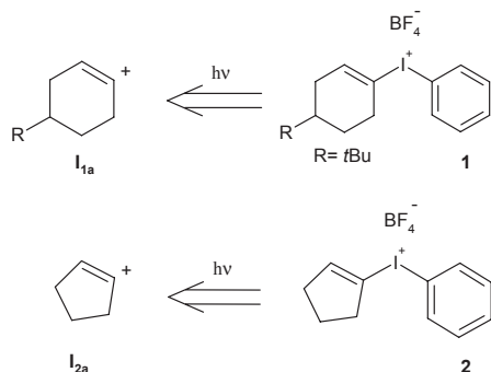
Chart 1: Cyclic vinyl cations produced from their corresponding iodonium salts.
