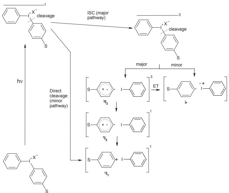
Scheme 8: Proposed mechanism of photolysis of diphenyliodonium salts.
