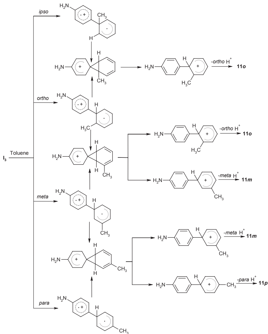
Scheme 5: Mechanism of product formation upon attack of the triplet 4-aminophenyl cation I_3\text{-NR}_2 on toluene.
