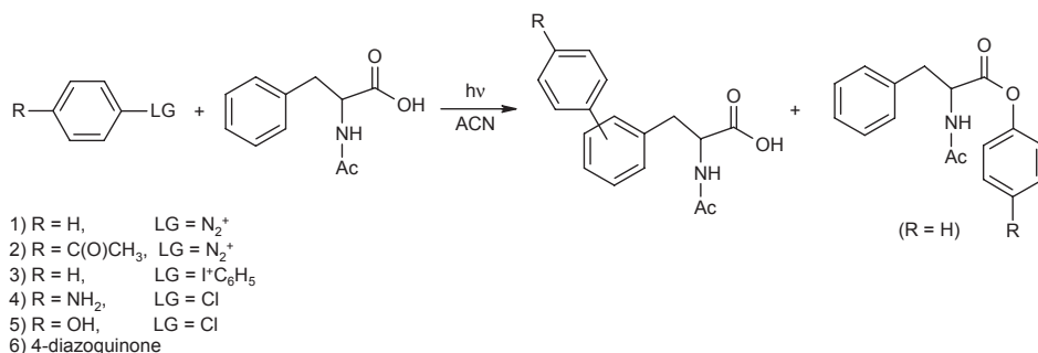
Scheme 3: Indicative photoreactions of a selection of aryl cation precursors with N-acetylated phenylalanine.
