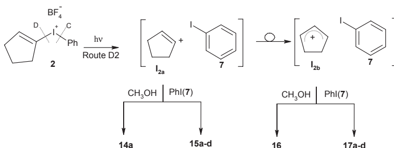
Scheme 4: Mechanism of formation of photoproducts 14–17 from 2 in methanol.
