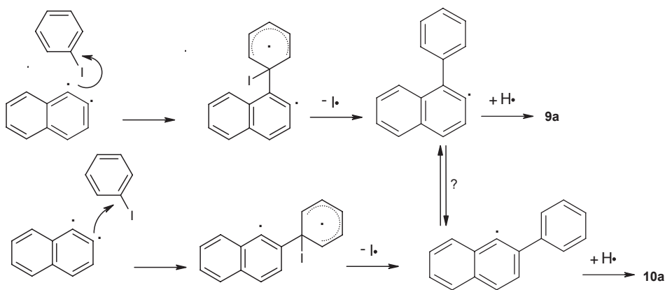
Scheme 8: Ipso-addition of iodobenzene to triplet naphthylene ^3\text{I}_8 , forming 9a and 10a .
