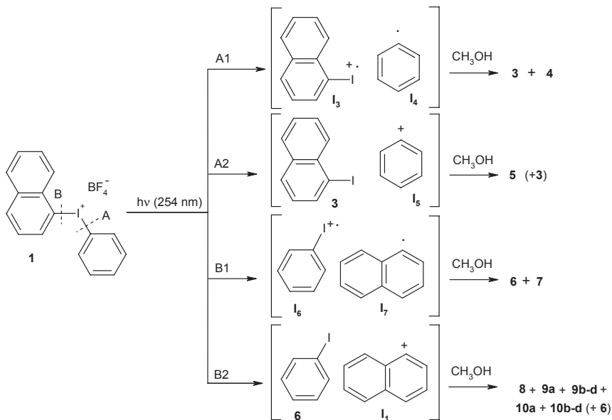
Scheme 2: Mechanism of product formation upon photolysis of 1 in methanol.
