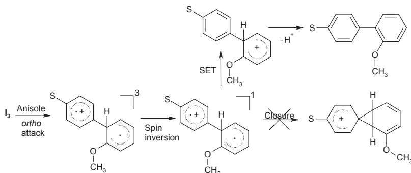
Scheme 5: Ortho attack of an EWG-substituted triplet phenyl cation ( I_3 ) on anisole ( S = \text{NO}_2 , \text{C}(=\text{O})\text{CH}_3 ).
