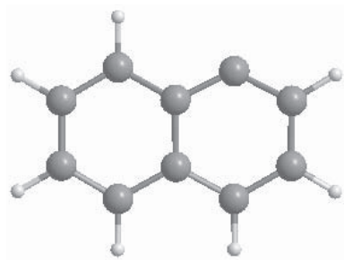
Cation ^3\text{I}_1 :
