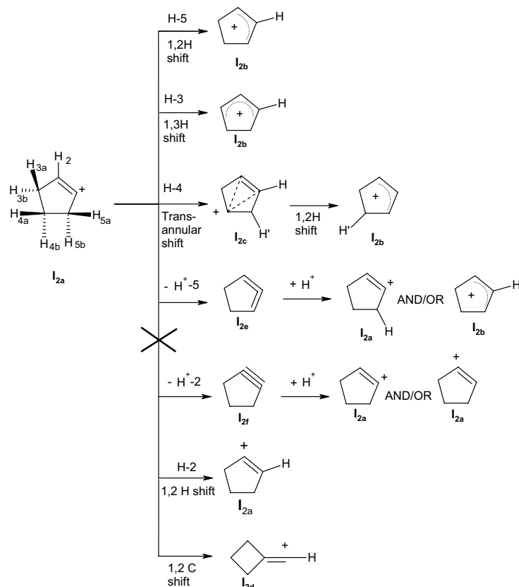
Scheme 6: Possible mechanisms of conversion of I_{2a} into I_{2b} .
