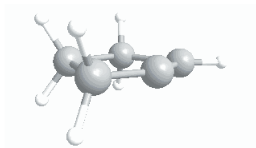
Vinyl cation I_{2a}
