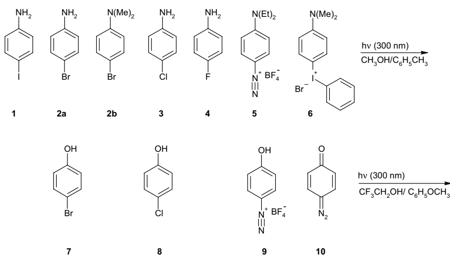
Chart 1: Compounds studied.
